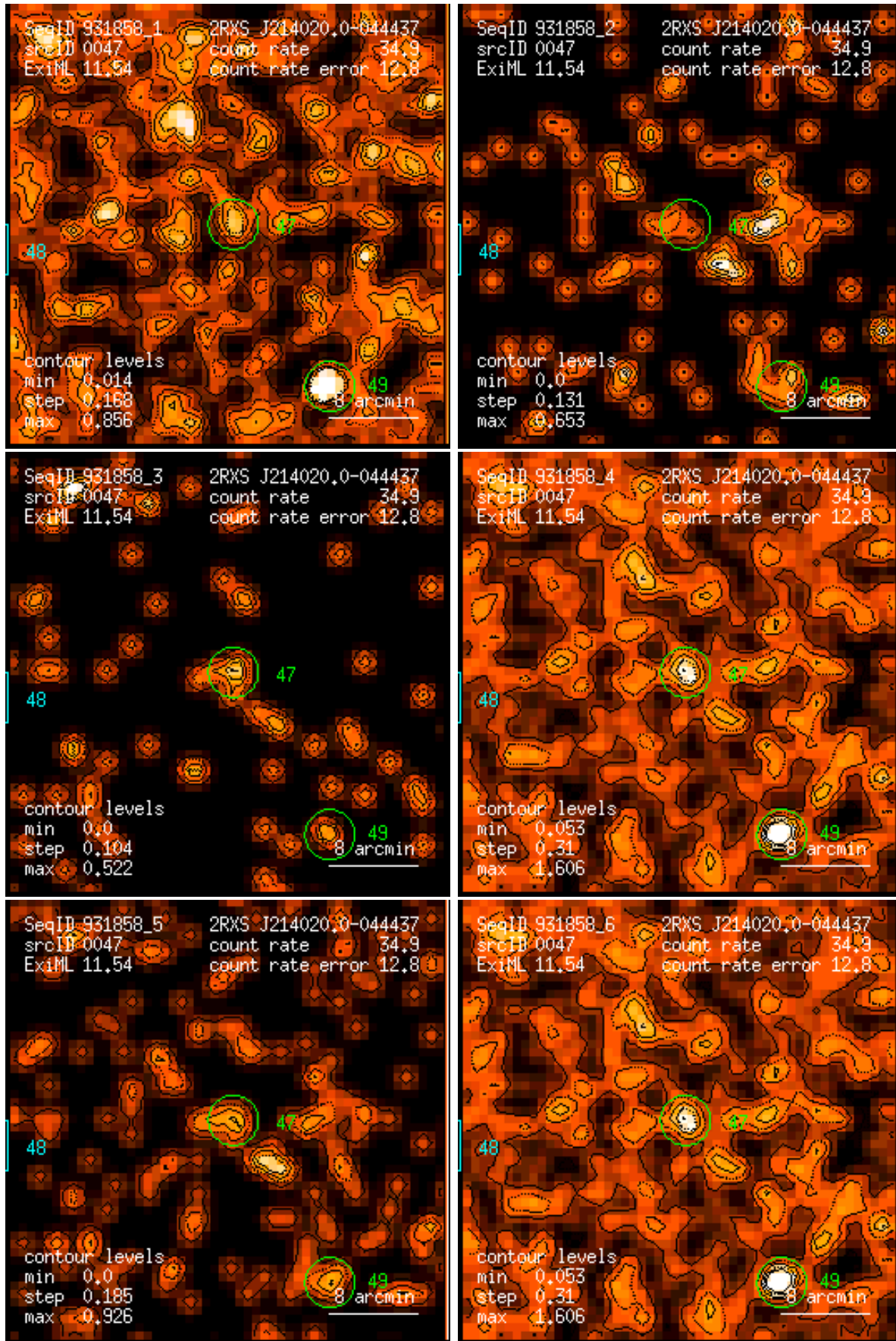
Figure 47: RASS 931858: detection 0047: band rate images, Gaussian filter: (1) PSPC channels 11 – 41, (2) 52 – 90, (3) 91 – 201, (4) 11 – 235, (5) 52 – 201, (6) 11 – 201. Broad band rates in counts/ks. Band rate contour levels in counts/ks/arcmin 2 .
