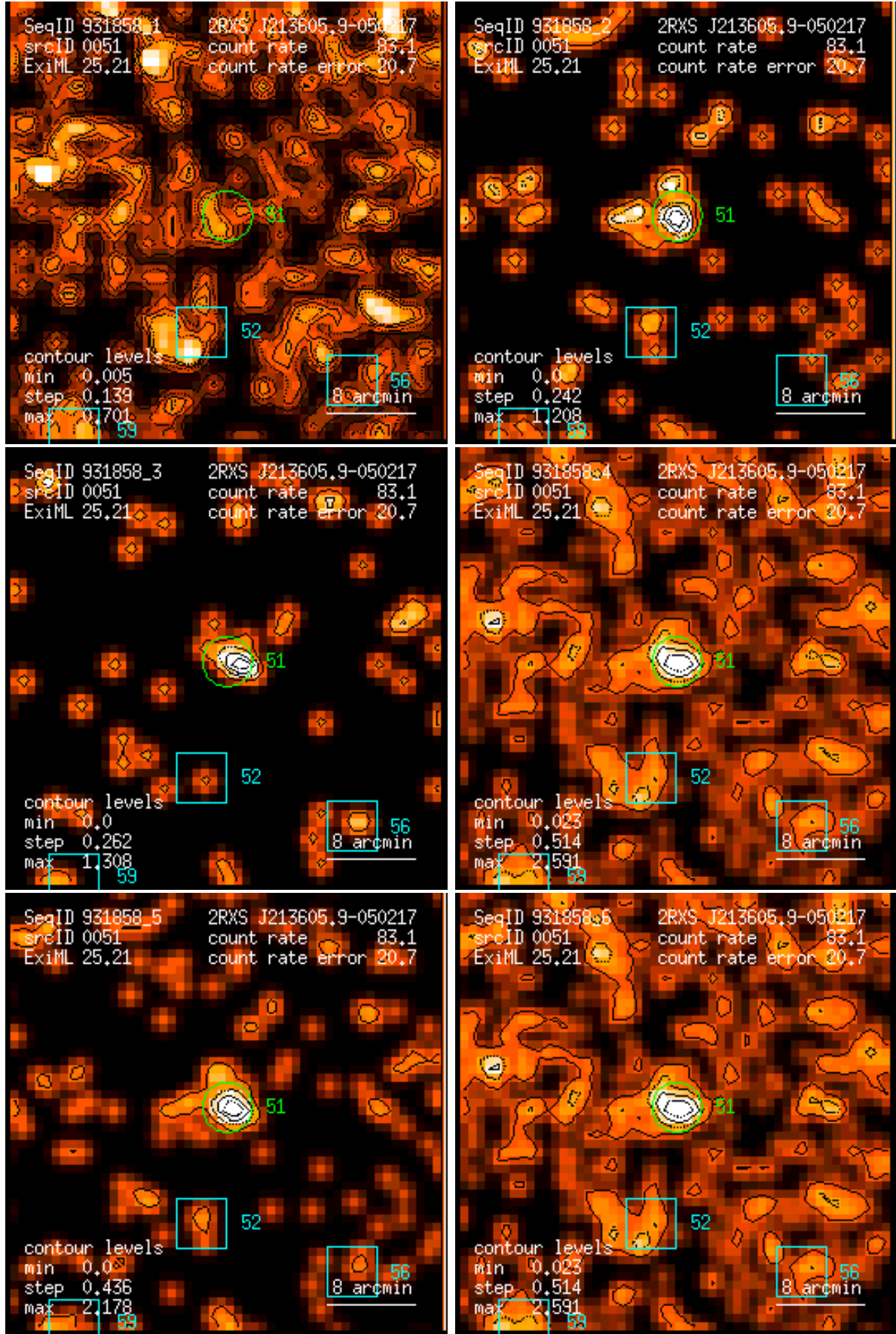
Figure 51: RASS 931858: detection 0051: band rate images, Gaussian filter: (1) PSPC channels 11 – 41, (2) 52 – 90, (3) 91 – 201, (4) 11 – 235, (5) 52 – 201, (6) 11 – 201. Broad band rates in counts/ks. Band rate contour levels in counts/ks/arcmin 2 .
