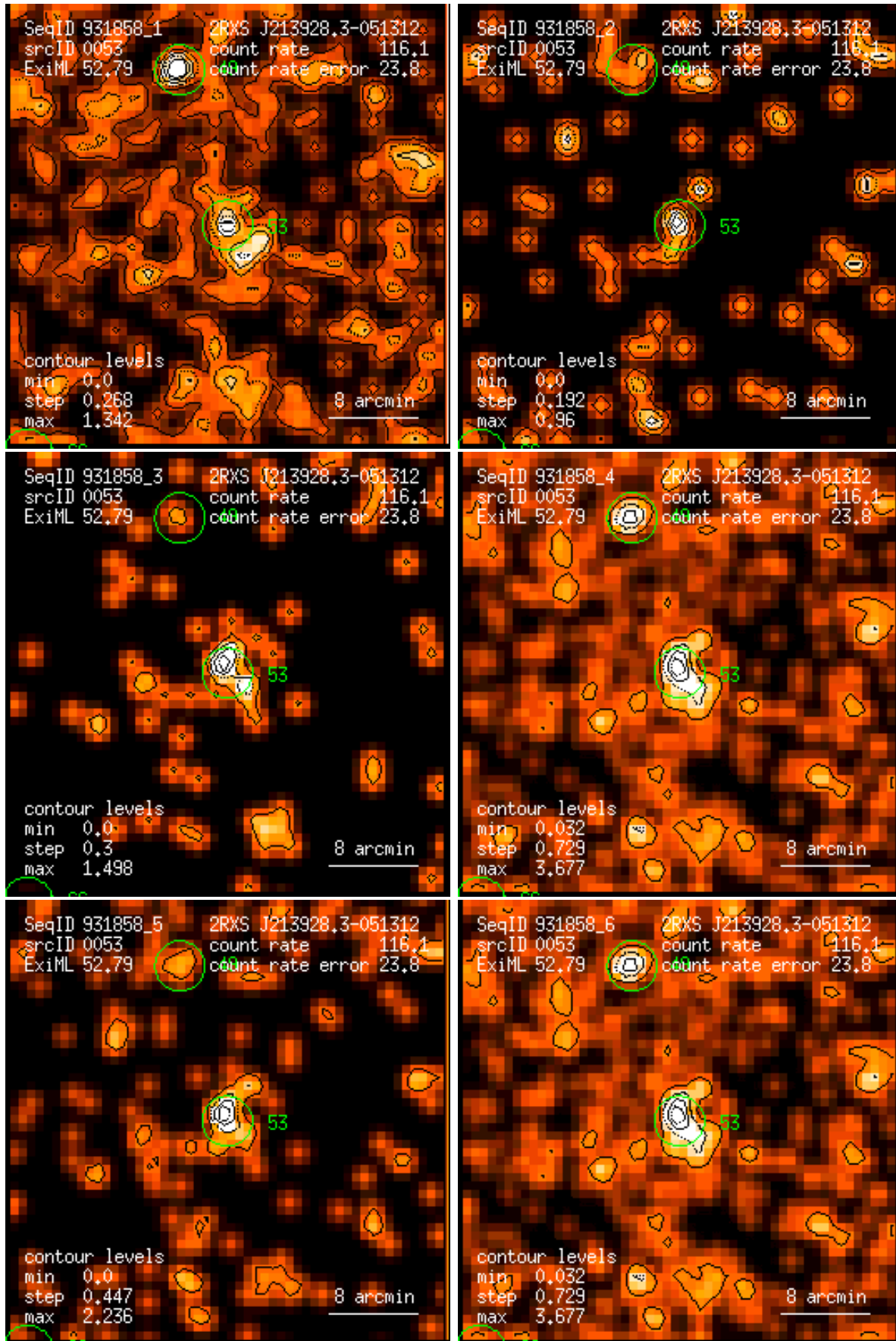
Figure 53: RASS 931858: detection 0053: band rate images, Gaussian filter: (1) PSPC channels 11 – 41, (2) 52 – 90, (3) 91 – 201, (4) 11 – 235, (5) 52 – 201, (6) 11 – 201. Broad band rates in counts/ks. Band rate contour levels in counts/ks/arcmin 2 .
