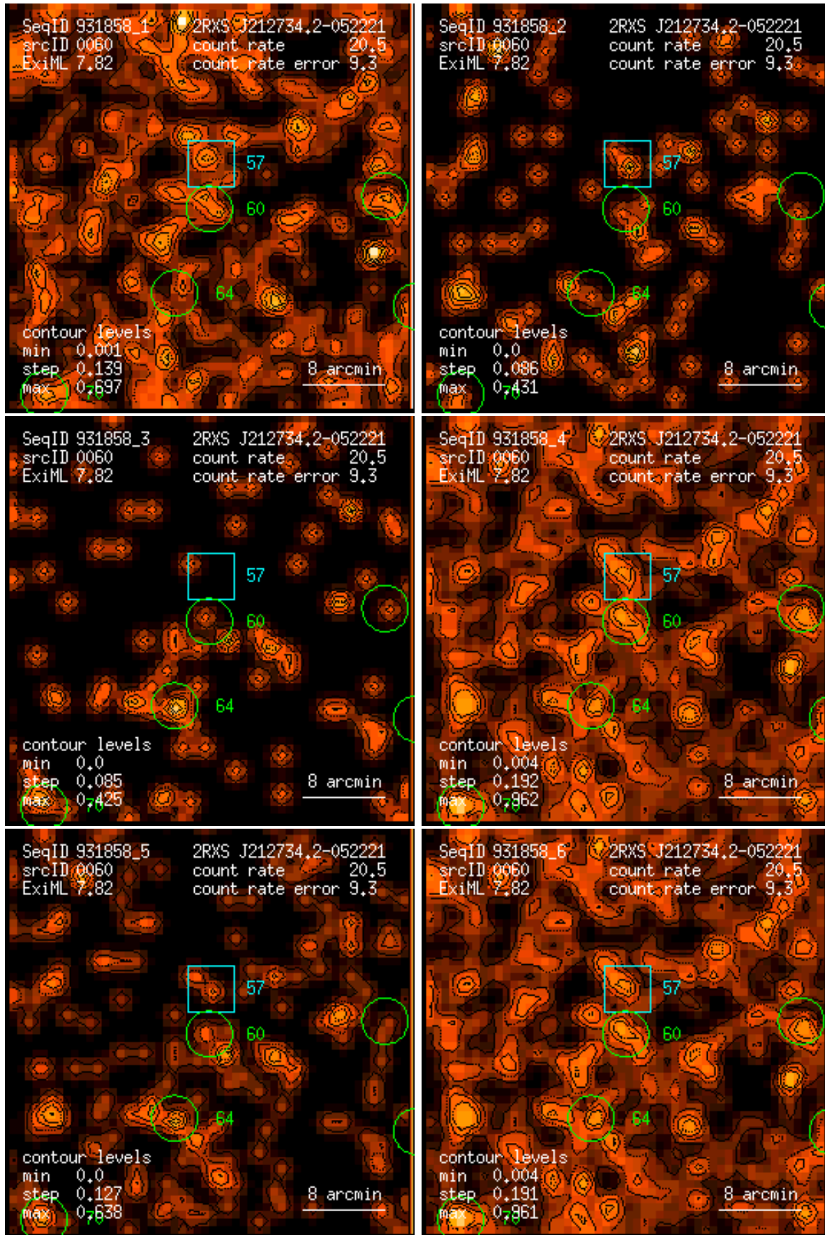
Figure 60: RASS 931858: detection 0060: band rate images, Gaussian filter: (1) PSPC channels 11 – 41, (2) 52 – 90, (3) 91 – 201, (4) 11 – 235, (5) 52 – 201, (6) 11 – 201. Broad band rates in counts/ks. Band rate contour levels in counts/ks/arcmin 2 .
