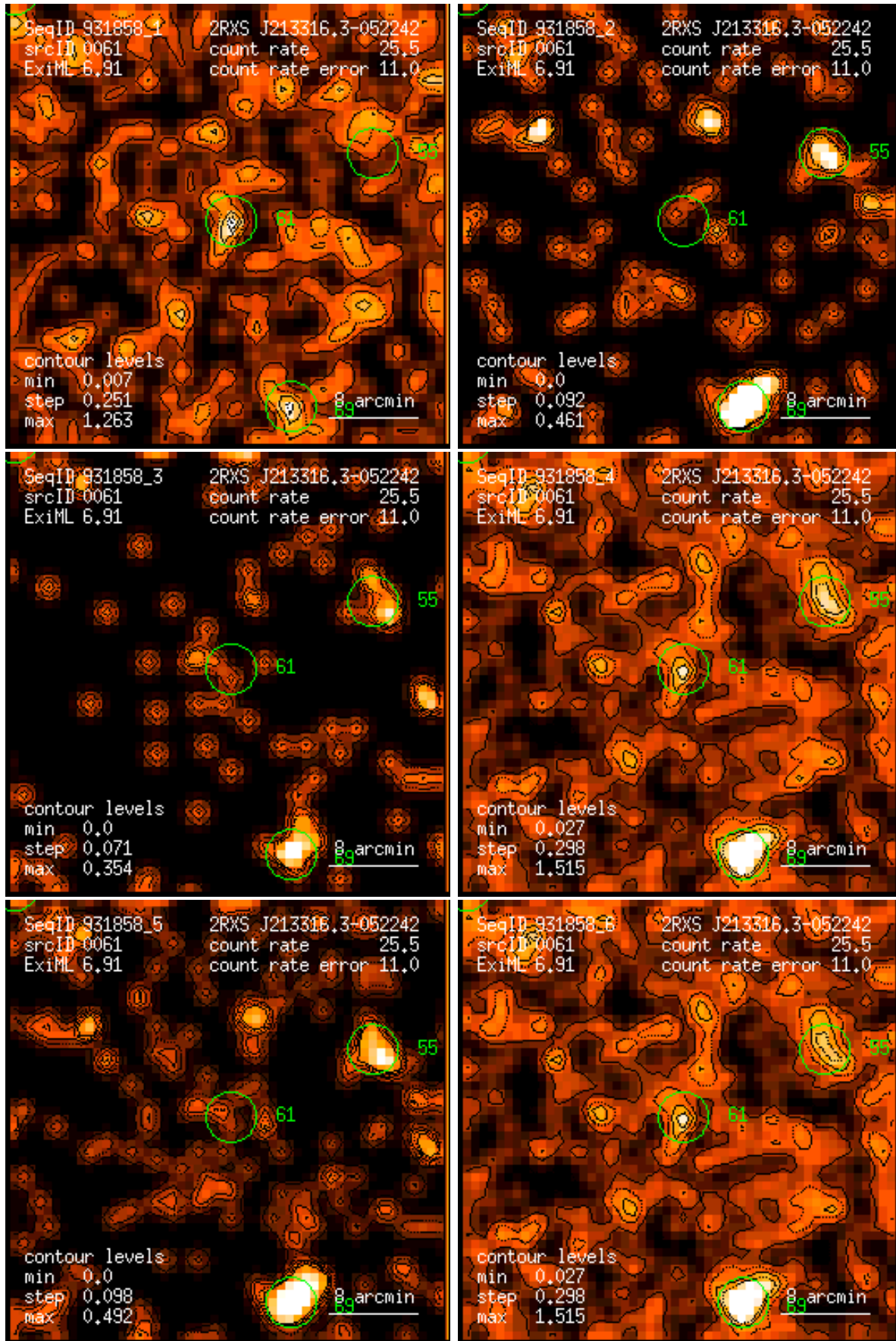
Figure 61: RASS 931858: detection 0061: band rate images, Gaussian filter: (1) PSPC channels 11 – 41, (2) 52 – 90, (3) 91 – 201, (4) 11 – 235, (5) 52 – 201, (6) 11 – 201. Broad band rates in counts/ks. Band rate contour levels in counts/ks/arcmin 2 .
