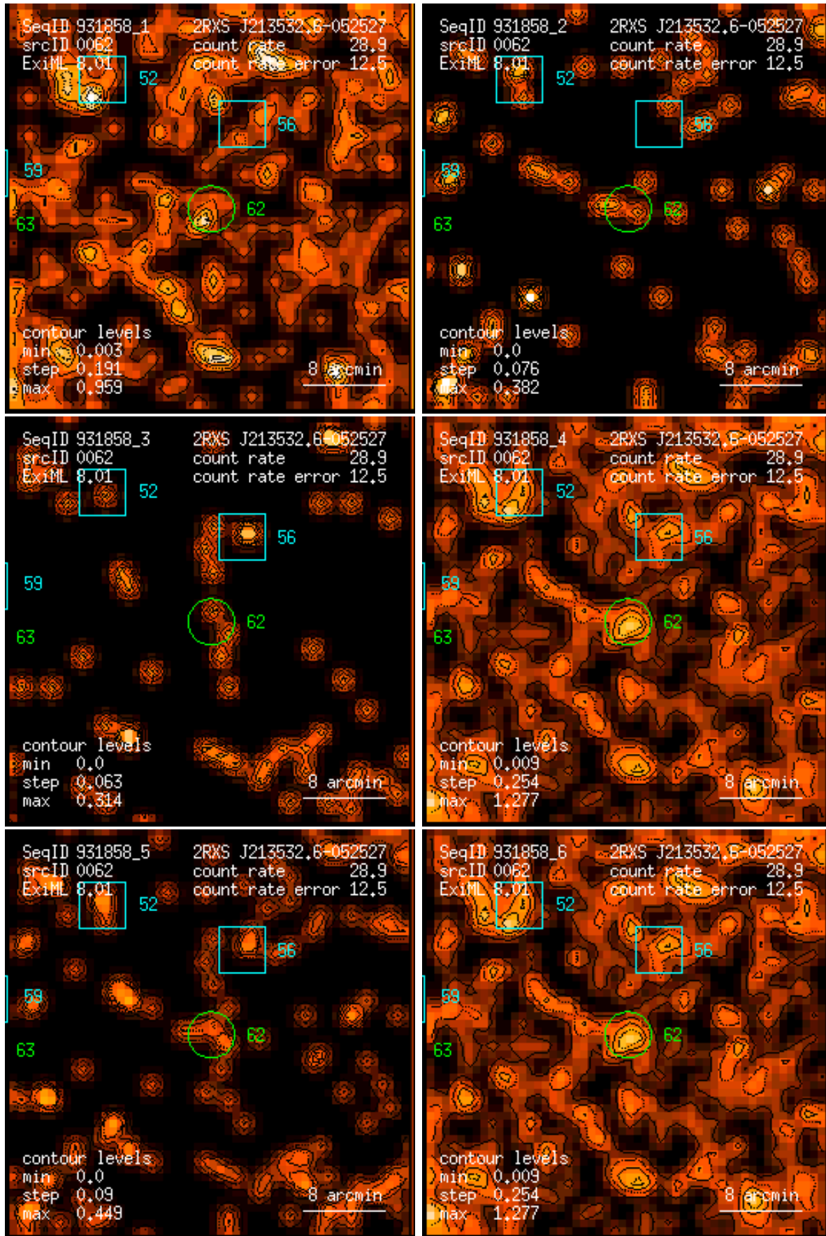
Figure 62: RASS 931858: detection 0062: band rate images, Gaussian filter: (1) PSPC channels 11 – 41, (2) 52 – 90, (3) 91 – 201, (4) 11 – 235, (5) 52 – 201, (6) 11 – 201. Broad band rates in counts/ks. Band rate contour levels in counts/ks/arcmin 2 .
