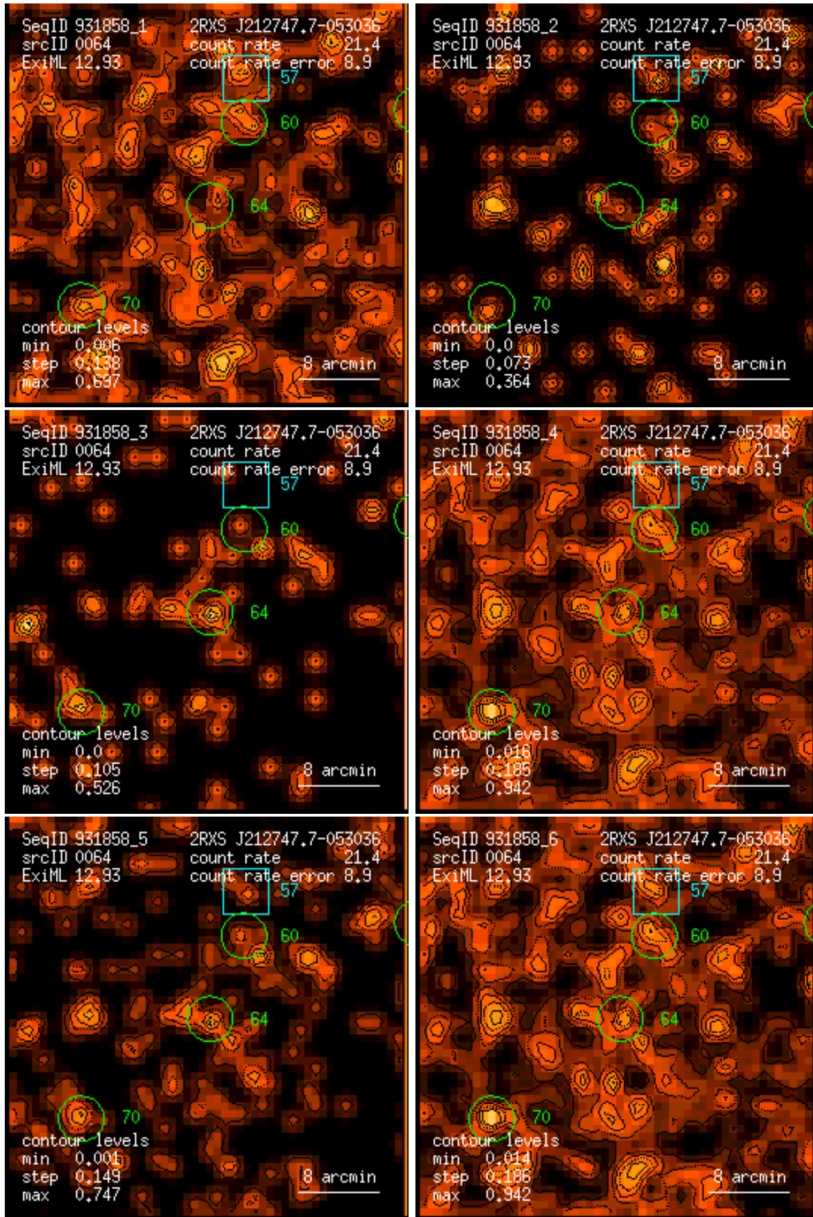
Figure 64: RASS 931858: detection 0064: band rate images, Gaussian filter: (1) PSPC channels 11 – 41, (2) 52 – 90, (3) 91 – 201, (4) 11 – 235, (5) 52 – 201, (6) 11 – 201. Broad band rates in counts/ks. Band rate contour levels in counts/ks/arcmin 2 .
