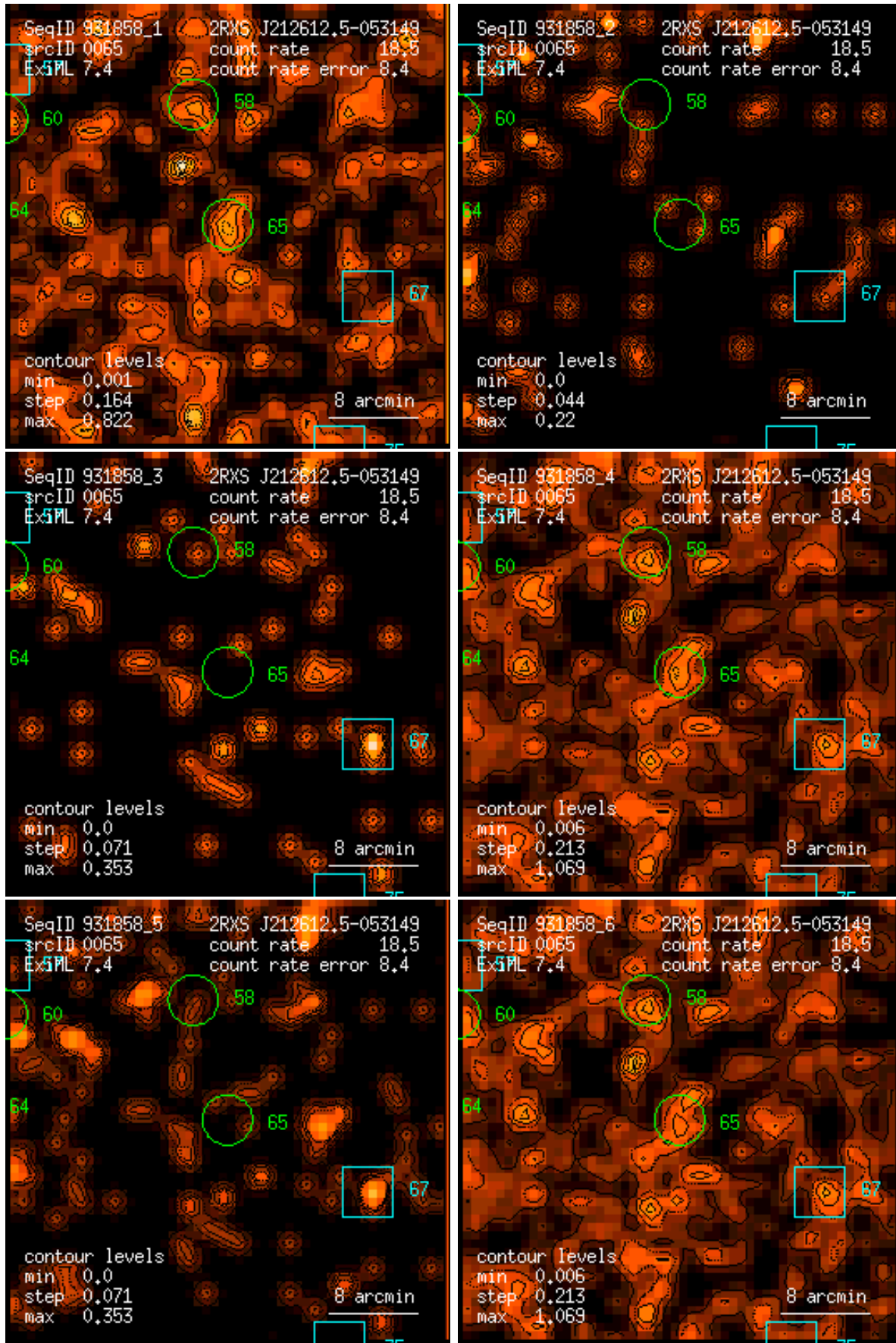
Figure 65: RASS 931858: detection 0065: band rate images, Gaussian filter: (1) PSPC channels 11 – 41, (2) 52 – 90, (3) 91 – 201, (4) 11 – 235, (5) 52 – 201, (6) 11 – 201. Broad band rates in counts/ks. Band rate contour levels in counts/ks/arcmin 2 .
