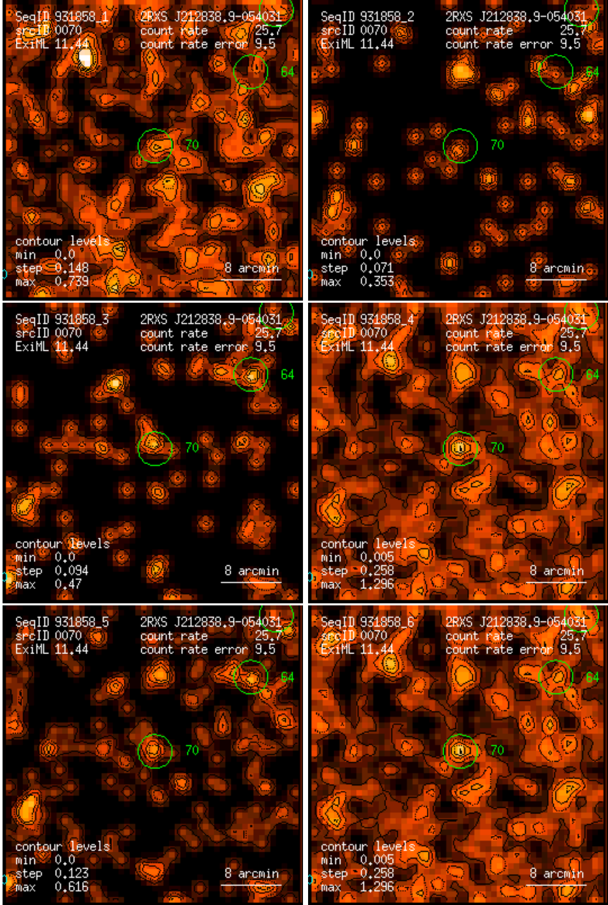
Figure 70: RASS 931858: detection 0070: band rate images, Gaussian filter: (1) PSPC channels 11 – 41, (2) 52 – 90, (3) 91 – 201, (4) 11 – 235, (5) 52 – 201, (6) 11 – 201. Broad band rates in counts/ks. Band rate contour levels in counts/ks/arcmin 2 .
