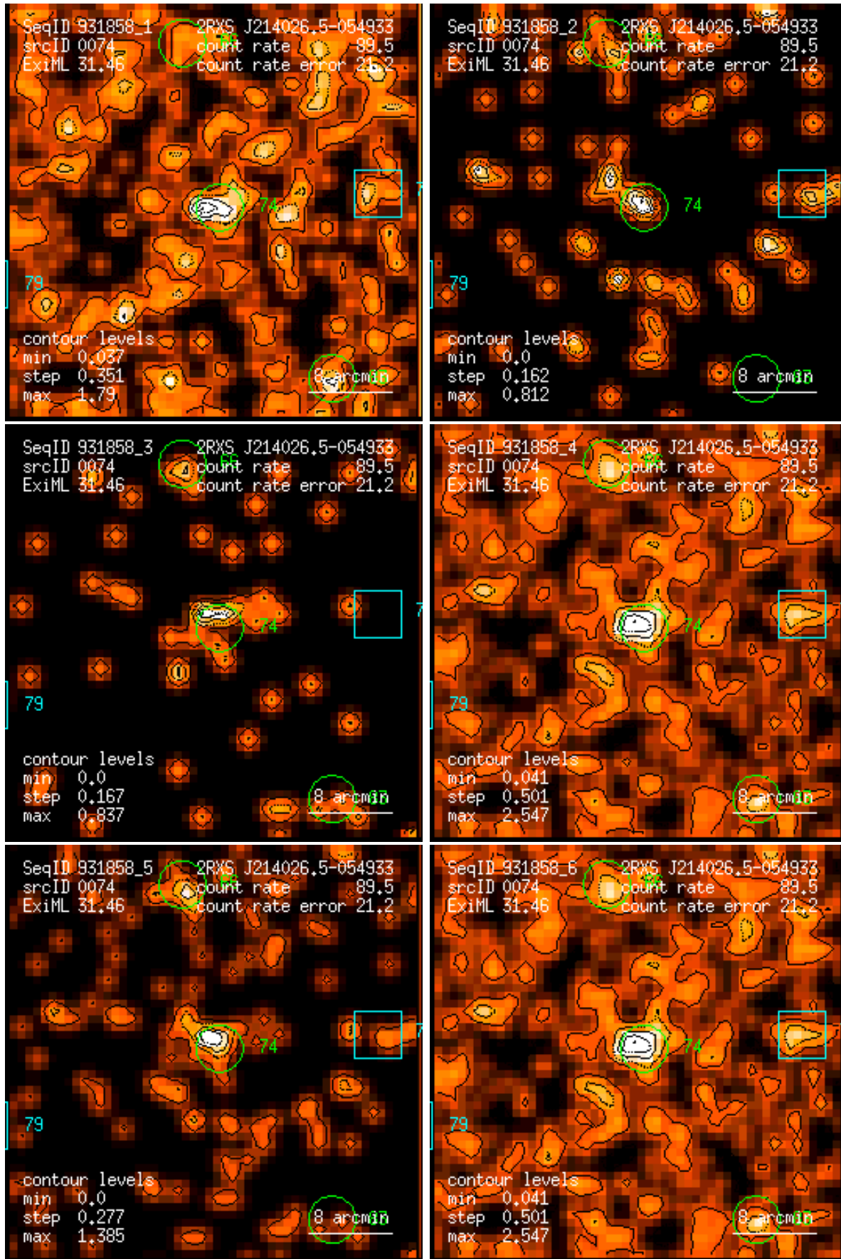
Figure 74: RASS 931858: detection 0074: band rate images, Gaussian filter: (1) PSPC channels 11 – 41, (2) 52 – 90, (3) 91 – 201, (4) 11 – 235, (5) 52 – 201, (6) 11 – 201. Broad band rates in counts/ks. Band rate contour levels in counts/ks/arcmin 2 .
