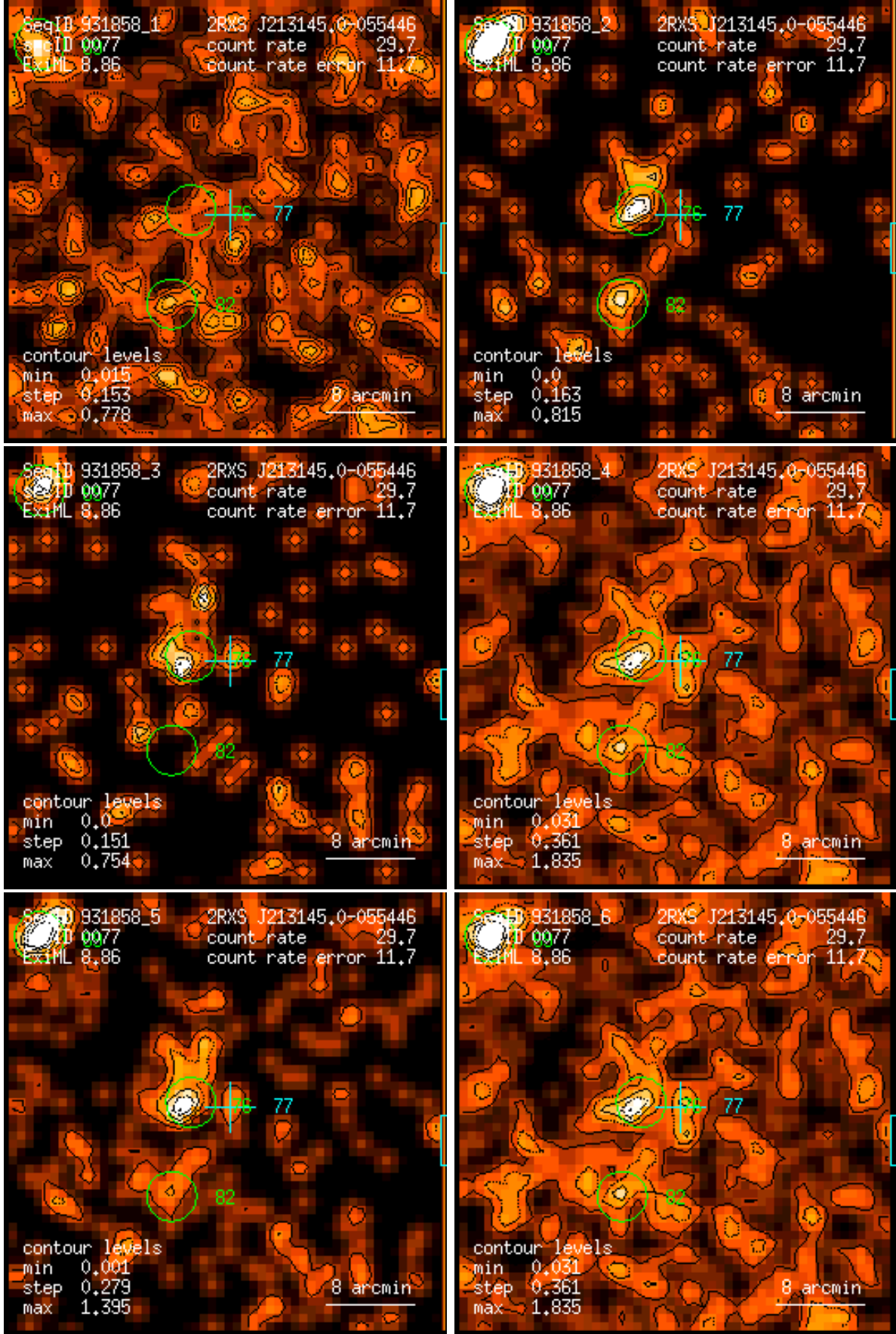
Figure 77: RASS 931858: detection 0077: band rate images, Gaussian filter: (1) PSPC channels 11 – 41, (2) 52 – 90, (3) 91 – 201, (4) 11 – 235, (5) 52 – 201, (6) 11 – 201. Broad band rates in counts/ks. Band rate contour levels in counts/ks/arcmin 2 .
