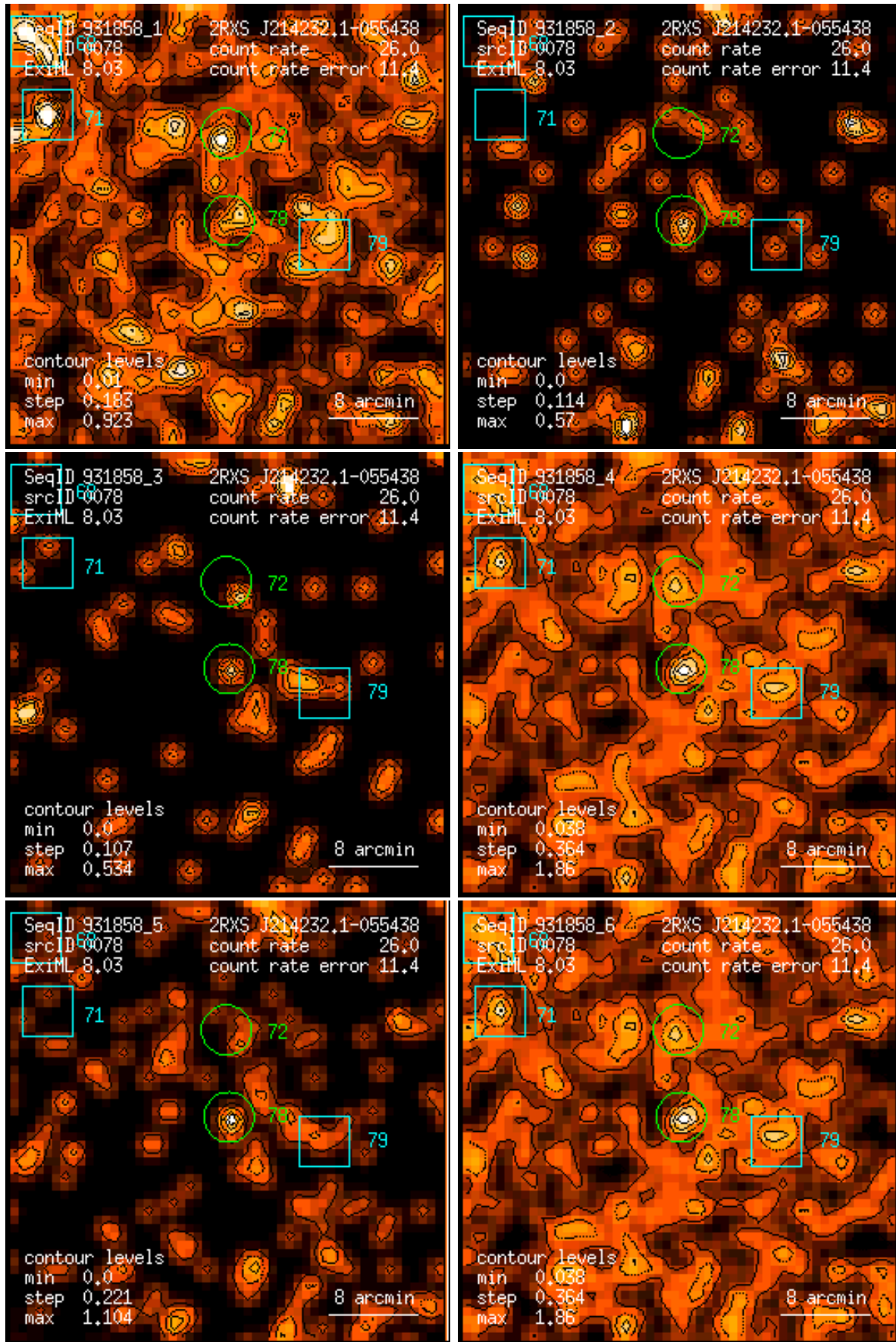
Figure 78: RASS 931858: detection 0078: band rate images, Gaussian filter: (1) PSPC channels 11 – 41, (2) 52 – 90, (3) 91 – 201, (4) 11 – 235, (5) 52 – 201, (6) 11 – 201. Broad band rates in counts/ks. Band rate contour levels in counts/ks/arcmin 2 .
