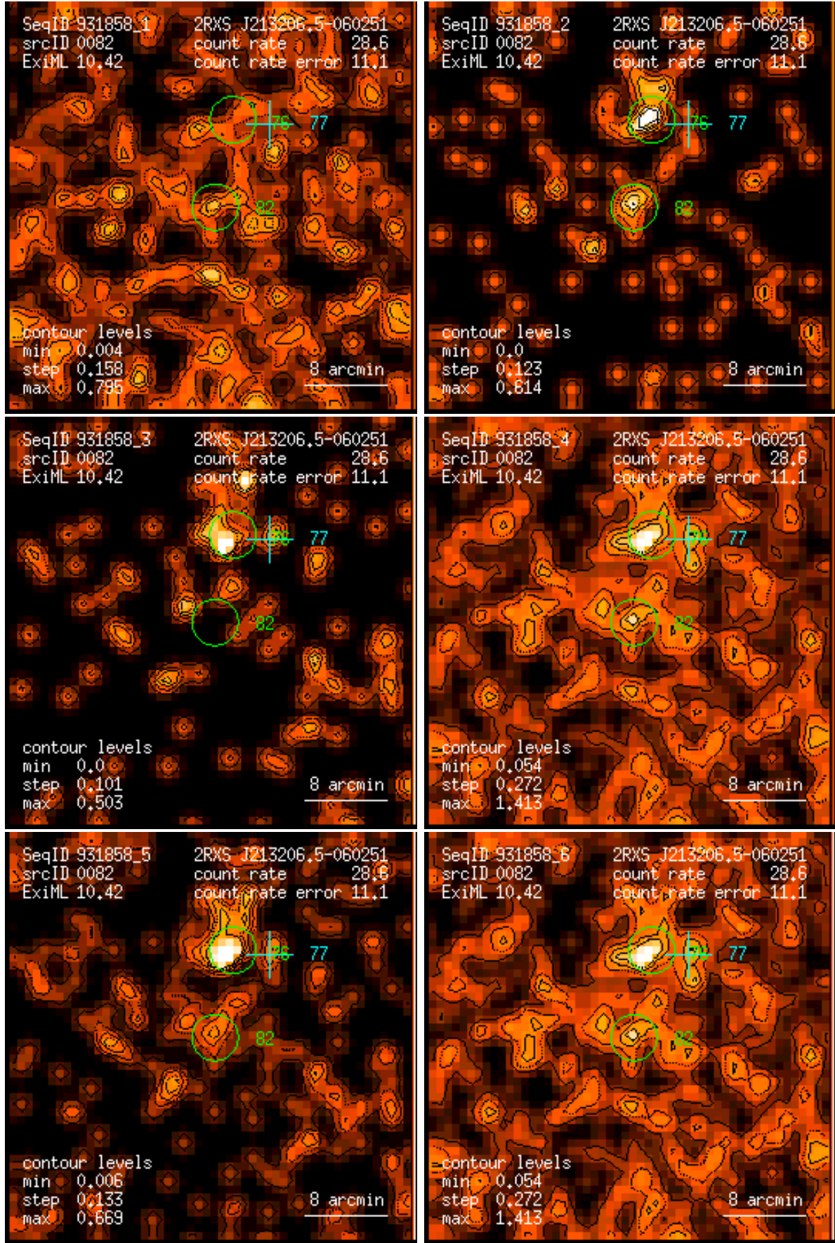
Figure 82: RASS 931858: detection 0082: band rate images, Gaussian filter: (1) PSPC channels 11 – 41, (2) 52 – 90, (3) 91 – 201, (4) 11 – 235, (5) 52 – 201, (6) 11 – 201. Broad band rates in counts/ks. Band rate contour levels in counts/ks/arcmin 2 .
