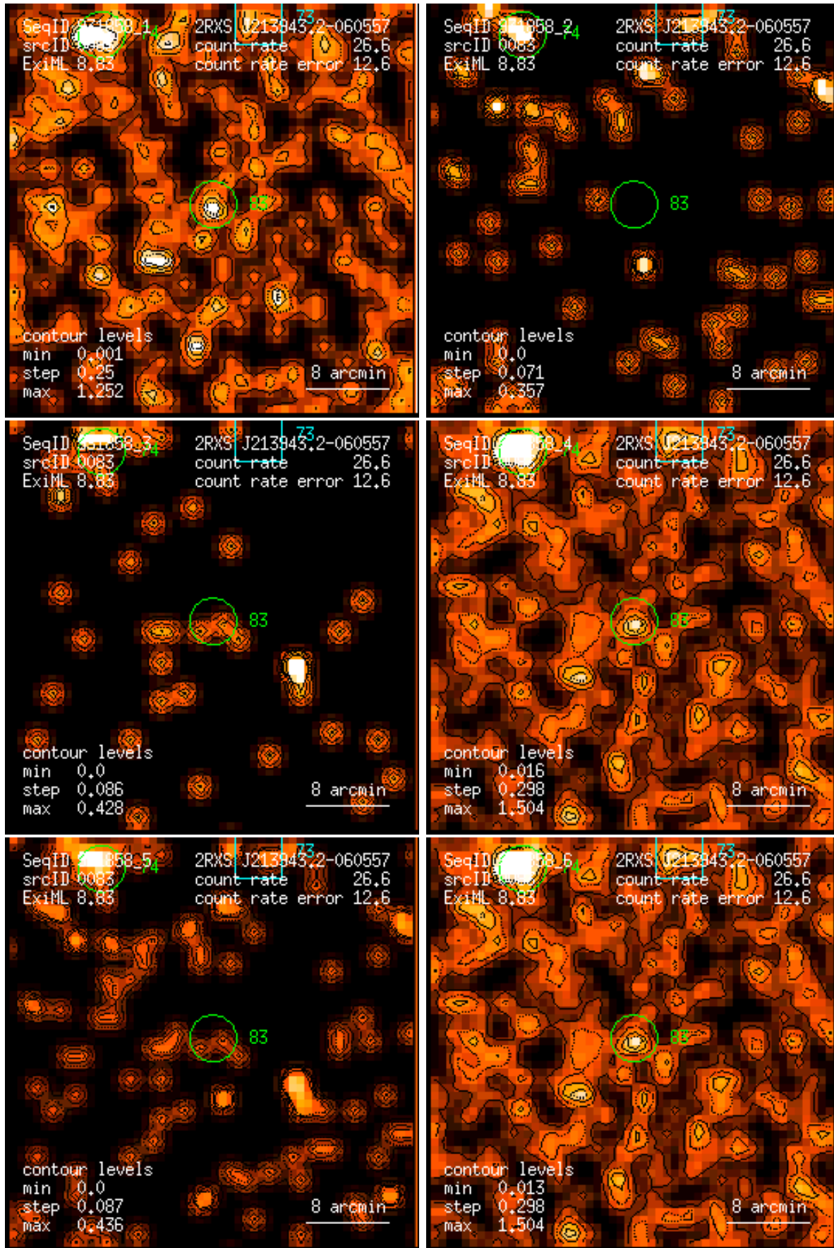
Figure 83: RASS 931858: detection 0083: band rate images, Gaussian filter: (1) PSPC channels 11 – 41, (2) 52 – 90, (3) 91 – 201, (4) 11 – 235, (5) 52 – 201, (6) 11 – 201. Broad band rates in counts/ks. Band rate contour levels in counts/ks/arcmin 2 .
