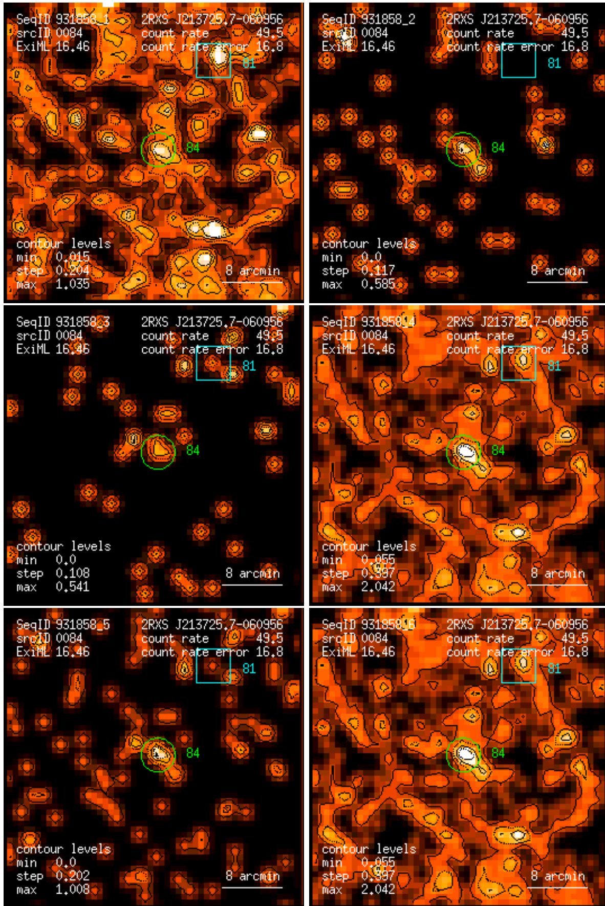
Figure 84: RASS 931858: detection 0084: band rate images, Gaussian filter: (1) PSPC channels 11 – 41, (2) 52 – 90, (3) 91 – 201, (4) 11 – 235, (5) 52 – 201, (6) 11 – 201. Broad band rates in counts/ks. Band rate contour levels in counts/ks/arcmin 2 .
