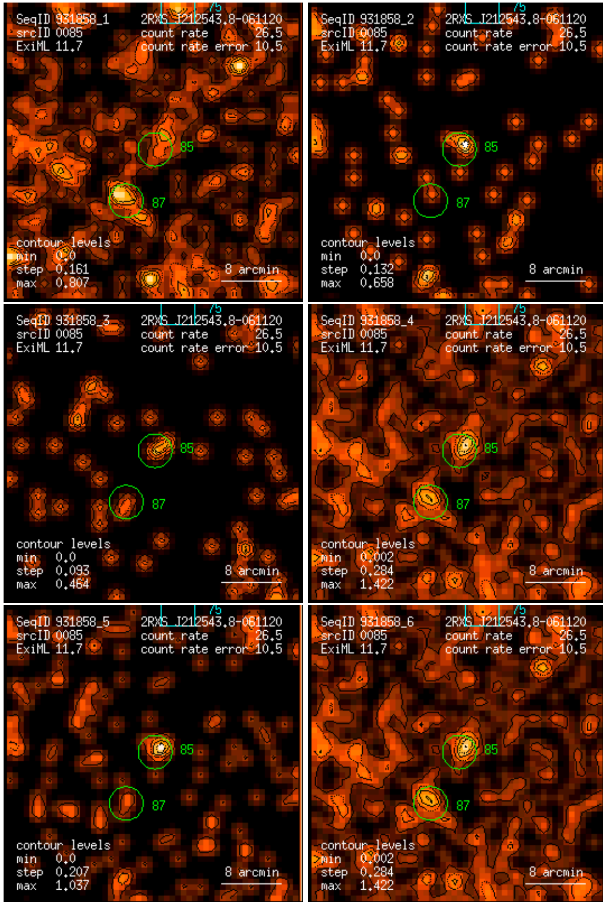
Figure 85: RASS 931858: detection 0085: band rate images, Gaussian filter: (1) PSPC channels 11 – 41, (2) 52 – 90, (3) 91 – 201, (4) 11 – 235, (5) 52 – 201, (6) 11 – 201. Broad band rates in counts/ks. Band rate contour levels in counts/ks/arcmin 2 .
