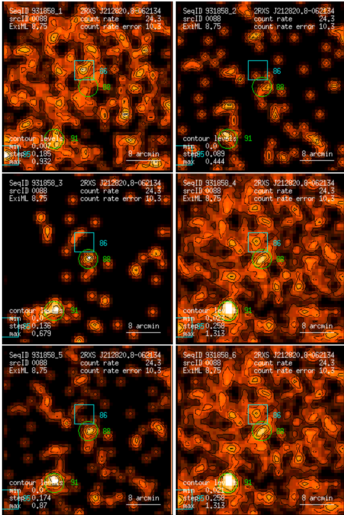
Figure 88: RASS 931858: detection 0088: band rate images, Gaussian filter: (1) PSPC channels 11 – 41, (2) 52 – 90, (3) 91 – 201, (4) 11 – 235, (5) 52 – 201, (6) 11 – 201. Broad band rates in counts/ks. Band rate contour levels in counts/ks/arcmin 2 .
