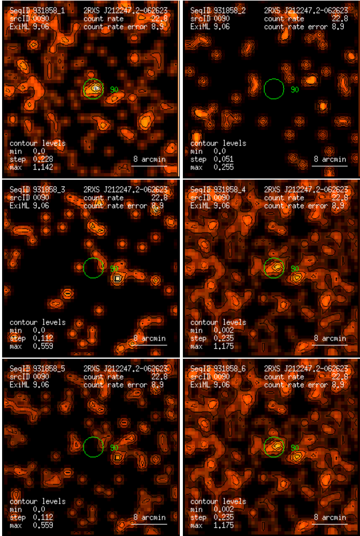
Figure 90: RASS 931858: detection 0090: band rate images, Gaussian filter: (1) PSPC channels 11 – 41, (2) 52 – 90, (3) 91 – 201, (4) 11 – 235, (5) 52 – 201, (6) 11 – 201. Broad band rates in counts/ks. Band rate contour levels in counts/ks/arcmin 2 .
