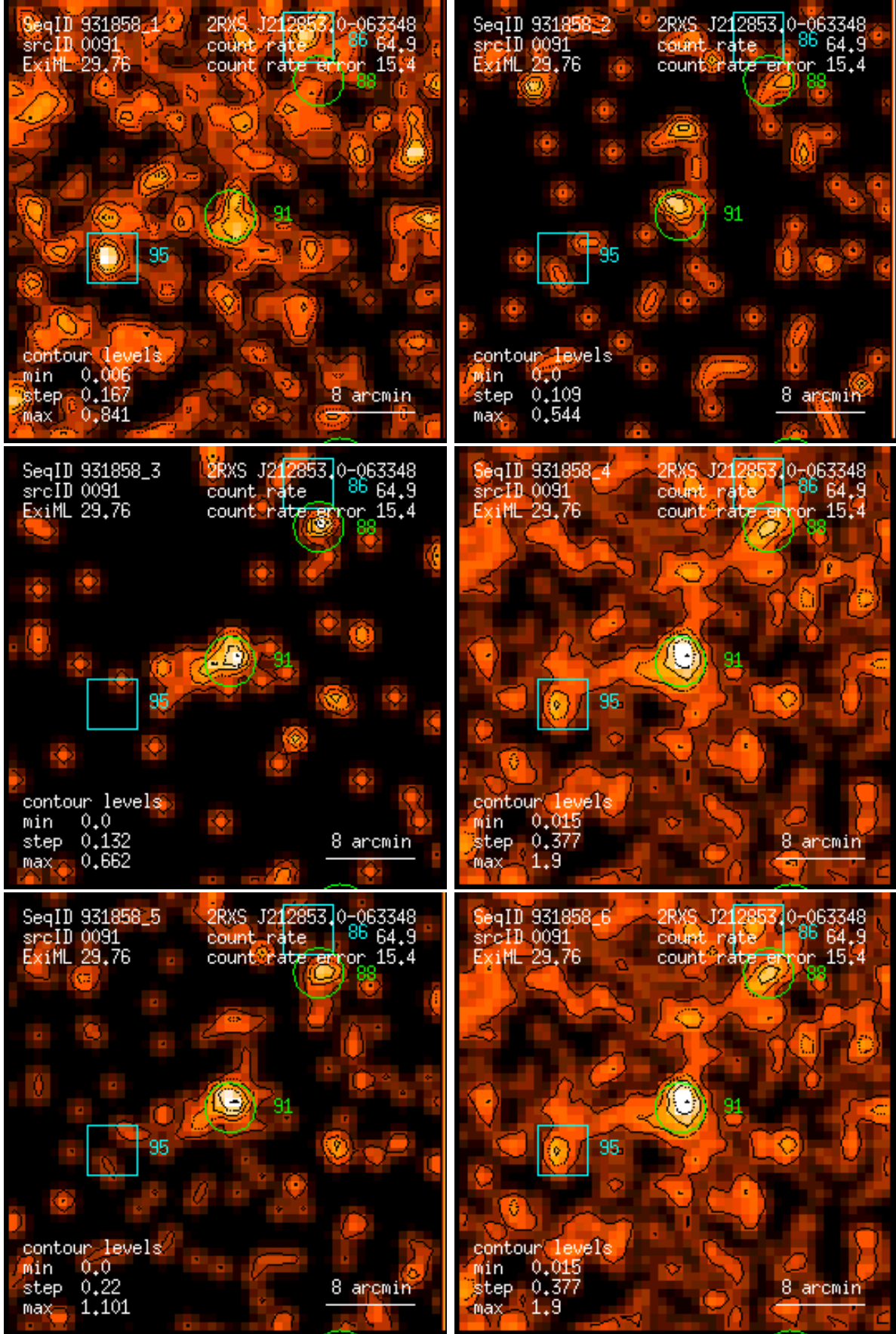
Figure 91: RASS 931858: detection 0091: band rate images, Gaussian filter: (1) PSPC channels 11 – 41, (2) 52 – 90, (3) 91 – 201, (4) 11 – 235, (5) 52 – 201, (6) 11 – 201. Broad band rates in counts/ks. Band rate contour levels in counts/ks/arcmin 2 .
