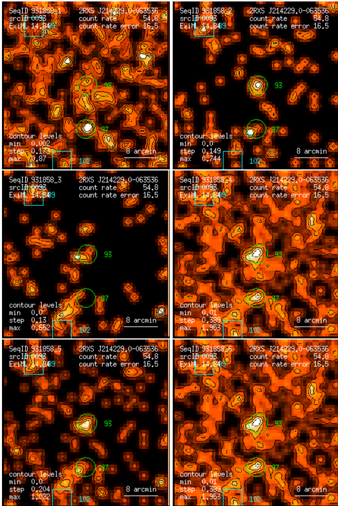
Figure 93: RASS 931858: detection 0093: band rate images, Gaussian filter: (1) PSPC channels 11 – 41, (2) 52 – 90, (3) 91 – 201, (4) 11 – 235, (5) 52 – 201, (6) 11 – 201. Broad band rates in counts/ks. Band rate contour levels in counts/ks/arcmin 2 .
