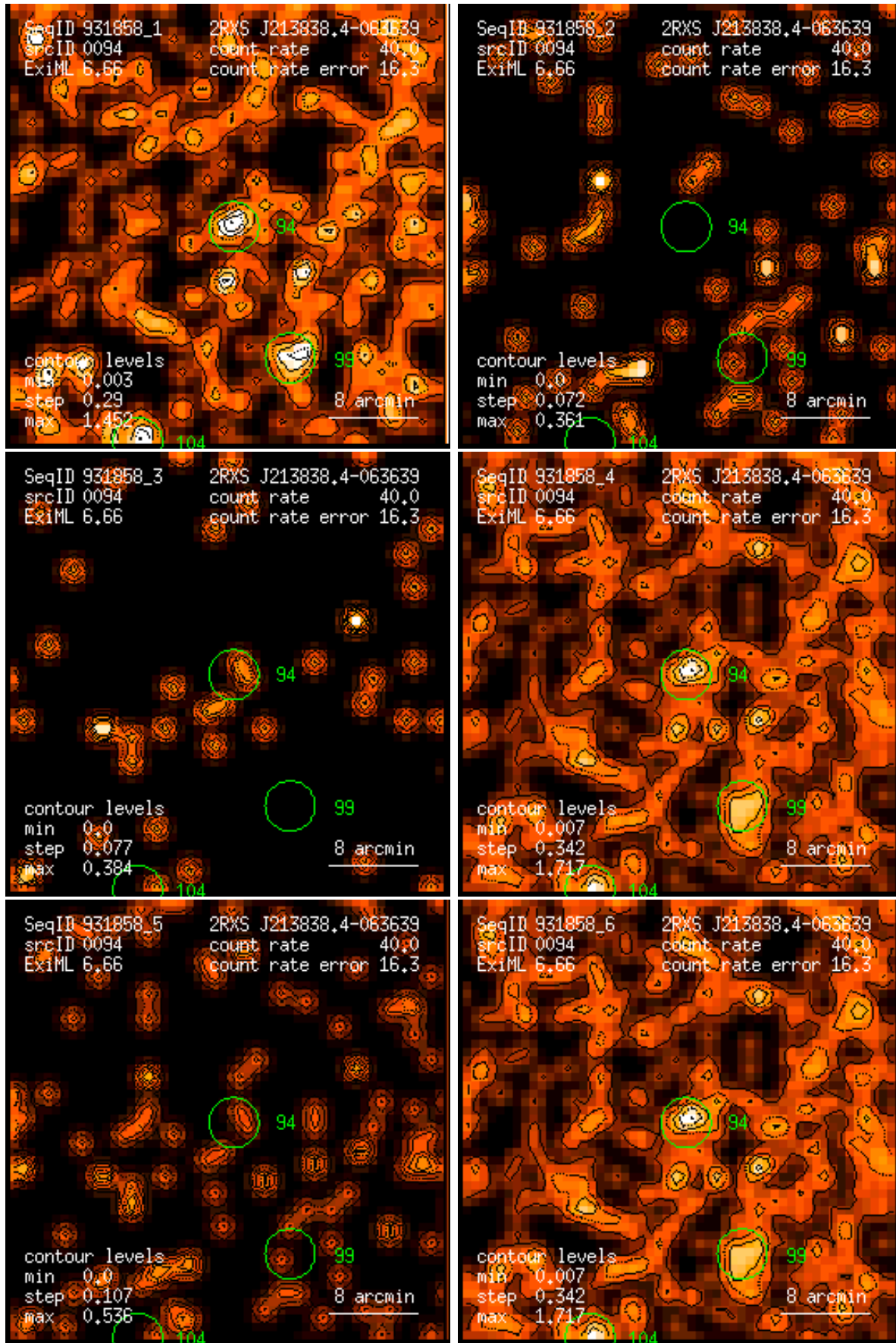
Figure 94: RASS 931858: detection 0094: band rate images, Gaussian filter: (1) PSPC channels 11 – 41, (2) 52 – 90, (3) 91 – 201, (4) 11 – 235, (5) 52 – 201, (6) 11 – 201. Broad band rates in counts/ks. Band rate contour levels in counts/ks/arcmin 2 .
