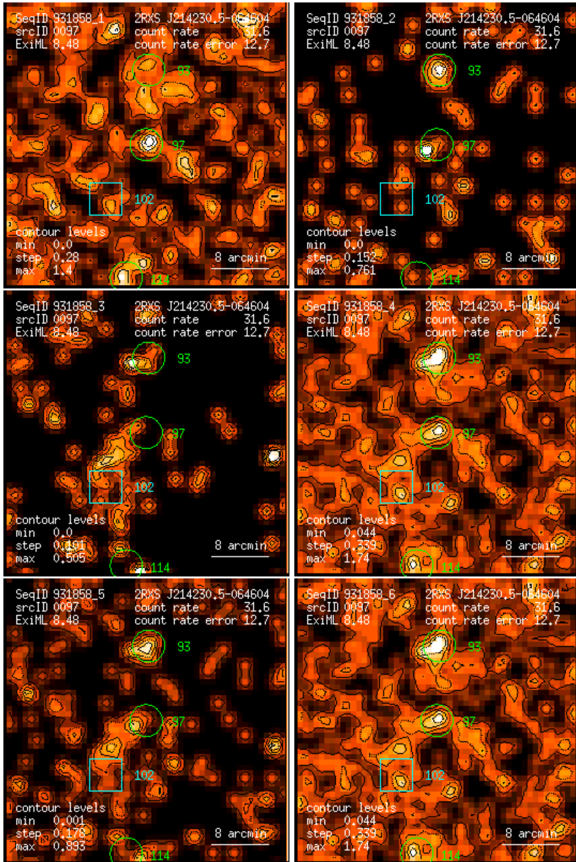
Figure 97: RASS 931858: detection 0097: band rate images, Gaussian filter: (1) PSPC channels 11 – 41, (2) 52 – 90, (3) 91 – 201, (4) 11 – 235, (5) 52 – 201, (6) 11 – 201. Broad band rates in counts/ks. Band rate contour levels in counts/ks/arcmin 2 .
