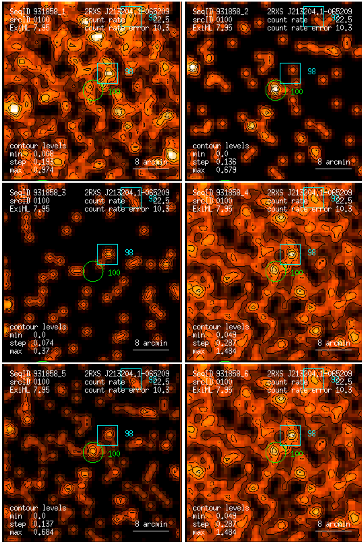
Figure 100: RASS 931858: detection 0100: band rate images, Gaussian filter: (1) PSPC channels 11 – 41, (2) 52 – 90, (3) 91 – 201, (4) 11 – 235, (5) 52 – 201, (6) 11 – 201. Broad band rates in counts/ks. Band rate contour levels in counts/ks/arcmin 2 .
