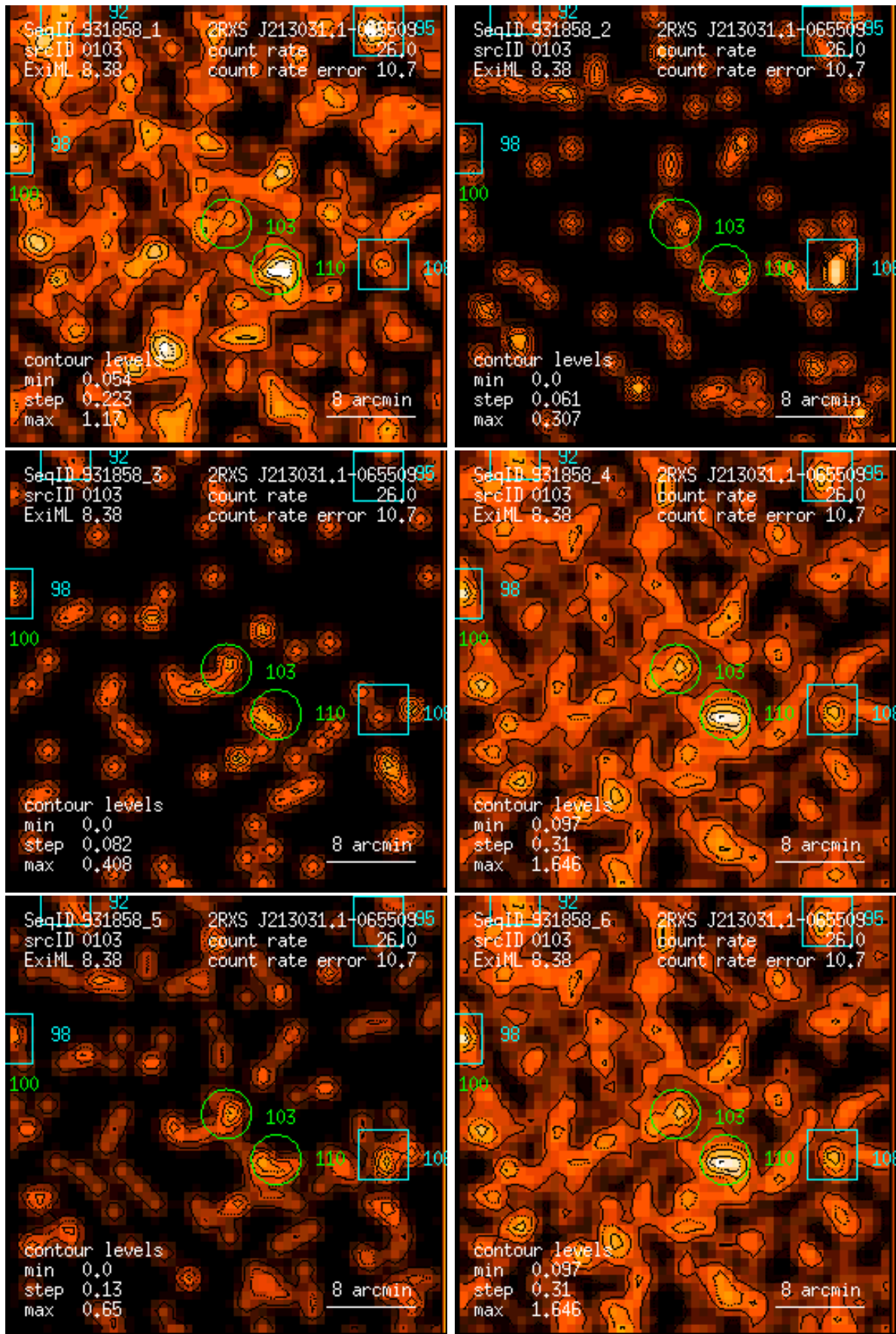
Figure 103: RASS 931858: detection 0103: band rate images, Gaussian filter: (1) PSPC channels 11 – 41, (2) 52 – 90, (3) 91 – 201, (4) 11 – 235, (5) 52 – 201, (6) 11 – 201. Broad band rates in counts/ks. Band rate contour levels in counts/ks/arcmin 2 .
