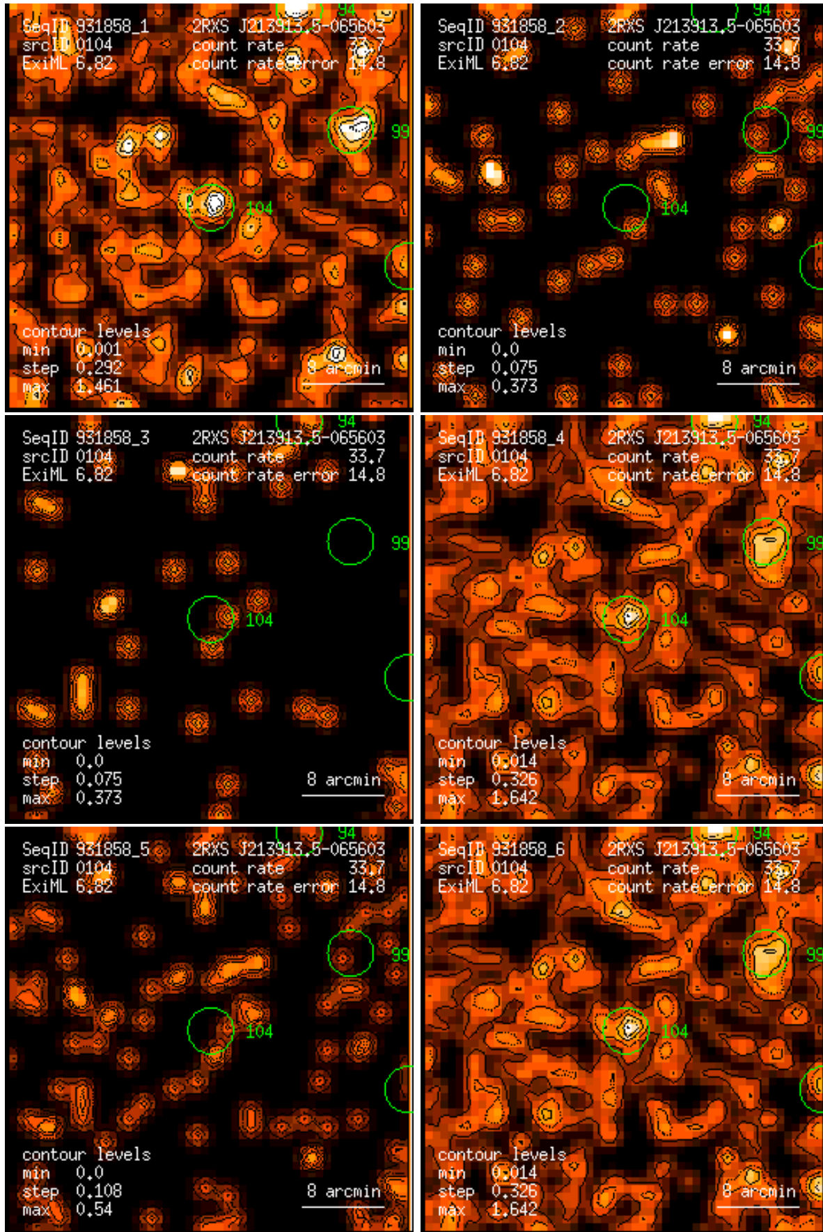
Figure 104: RASS 931858: detection 0104: band rate images, Gaussian filter: (1) PSPC channels 11 – 41, (2) 52 – 90, (3) 91 – 201, (4) 11 – 235, (5) 52 – 201, (6) 11 – 201. Broad band rates in counts/ks. Band rate contour levels in counts/ks/arcmin 2 .
