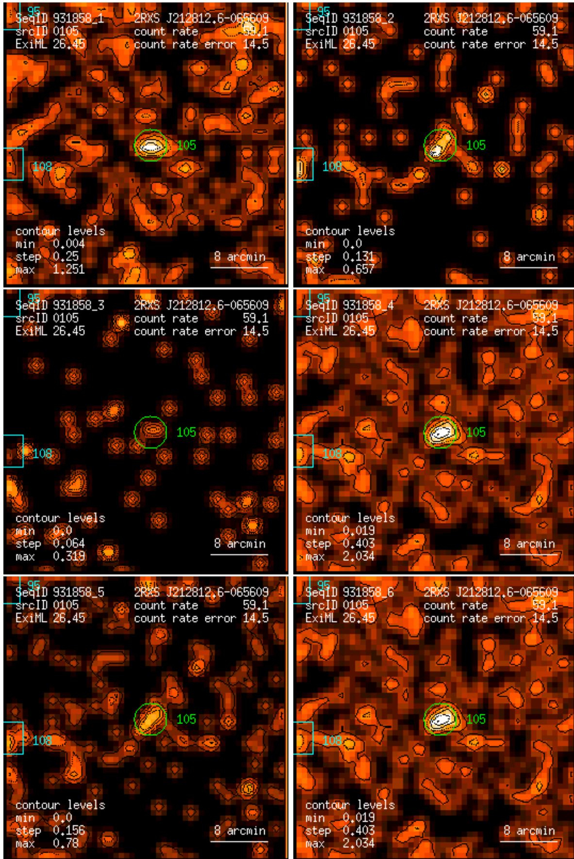
Figure 105: RASS 931858: detection 0105: band rate images, Gaussian filter: (1) PSPC channels 11 – 41, (2) 52 – 90, (3) 91 – 201, (4) 11 – 235, (5) 52 – 201, (6) 11 – 201. Broad band rates in counts/ks. Band rate contour levels in counts/ks/arcmin 2 .
