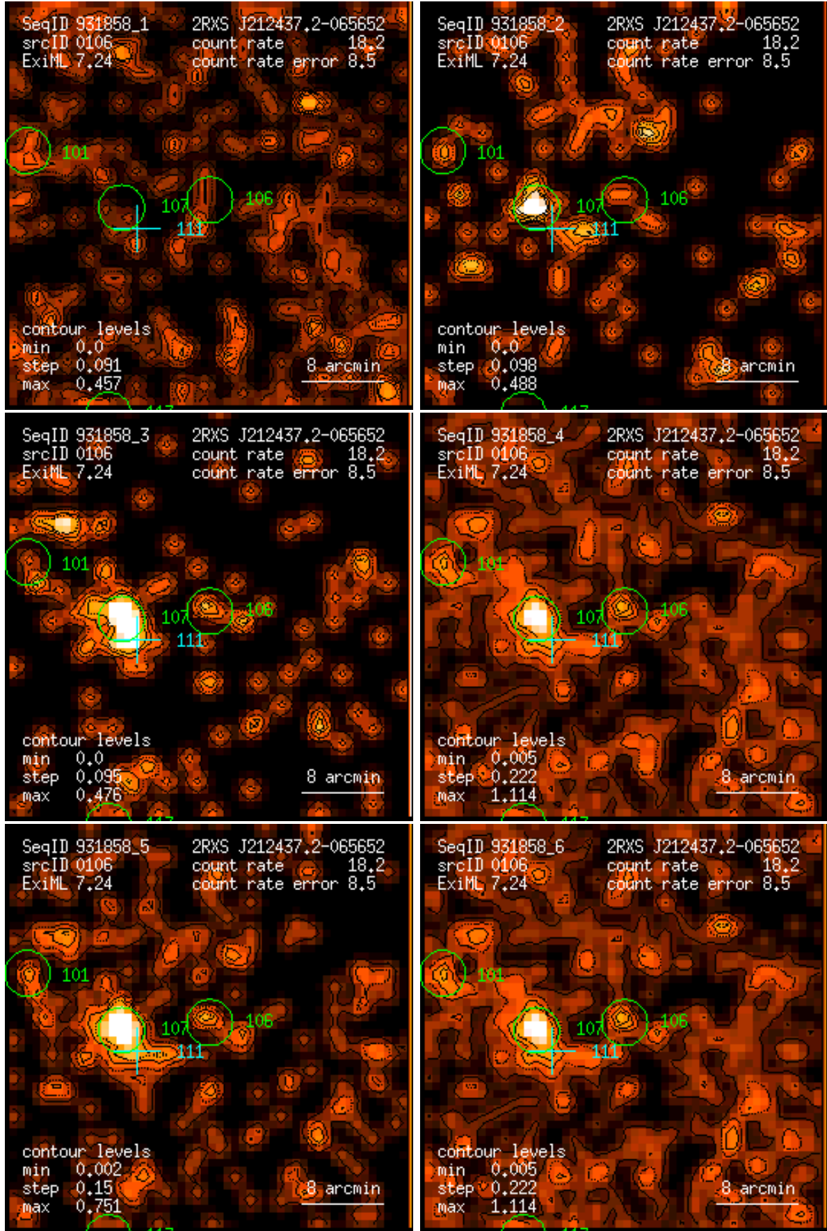
Figure 106: RASS 931858: detection 0106: band rate images, Gaussian filter: (1) PSPC channels 11 – 41, (2) 52 – 90, (3) 91 – 201, (4) 11 – 235, (5) 52 – 201, (6) 11 – 201. Broad band rates in counts/ks. Band rate contour levels in counts/ks/arcmin 2 .
