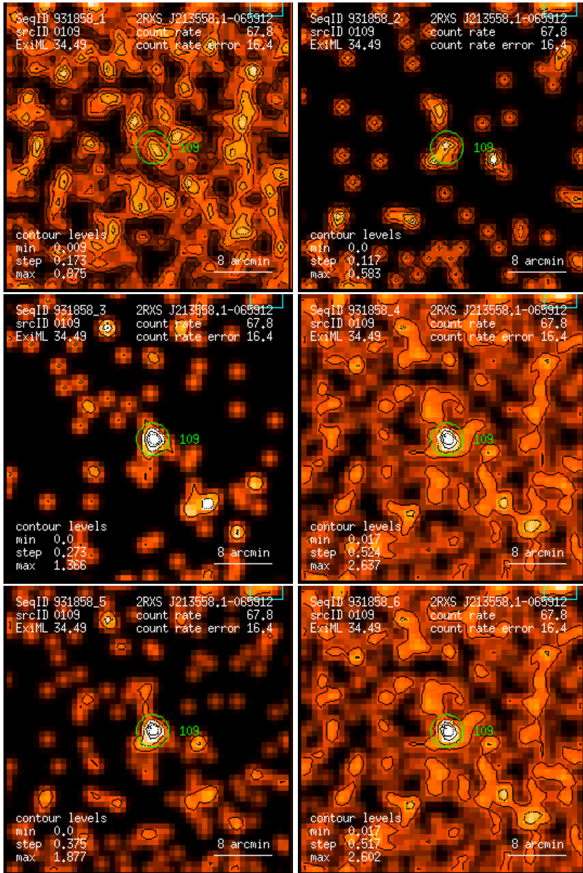
Figure 109: RASS 931858: detection 0109: band rate images, Gaussian filter: (1) PSPC channels 11 – 41, (2) 52 – 90, (3) 91 – 201, (4) 11 – 235, (5) 52 – 201, (6) 11 – 201. Broad band rates in counts/ks. Band rate contour levels in counts/ks/arcmin 2 .
