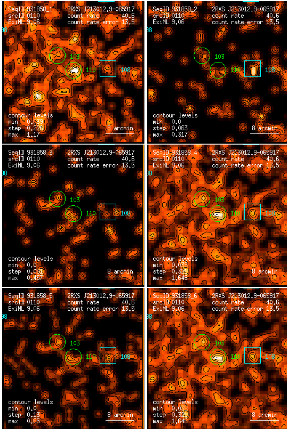
Figure 110: RASS 931858: detection 0110: band rate images, Gaussian filter: (1) PSPC channels 11 – 41, (2) 52 – 90, (3) 91 – 201, (4) 11 – 235, (5) 52 – 201, (6) 11 – 201. Broad band rates in counts/ks. Band rate contour levels in counts/ks/arcmin 2 .
