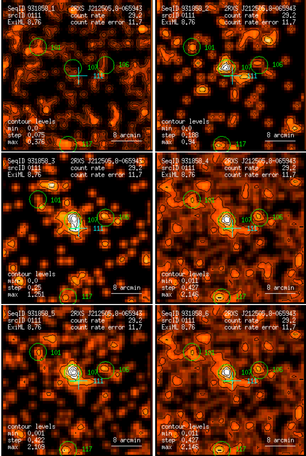
Figure 111: RASS 931858: detection 0111: band rate images, Gaussian filter: (1) PSPC channels 11 – 41, (2) 52 – 90, (3) 91 – 201, (4) 11 – 235, (5) 52 – 201, (6) 11 – 201. Broad band rates in counts/ks. Band rate contour levels in counts/ks/arcmin 2 .
