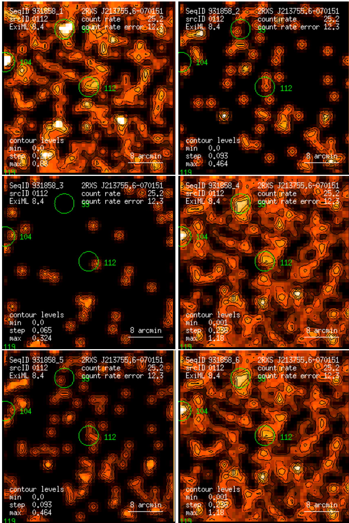
Figure 112: RASS 931858: detection 0112: band rate images, Gaussian filter: (1) PSPC channels 11 – 41, (2) 52 – 90, (3) 91 – 201, (4) 11 – 235, (5) 52 – 201, (6) 11 – 201. Broad band rates in counts/ks. Band rate contour levels in counts/ks/arcmin 2 .
