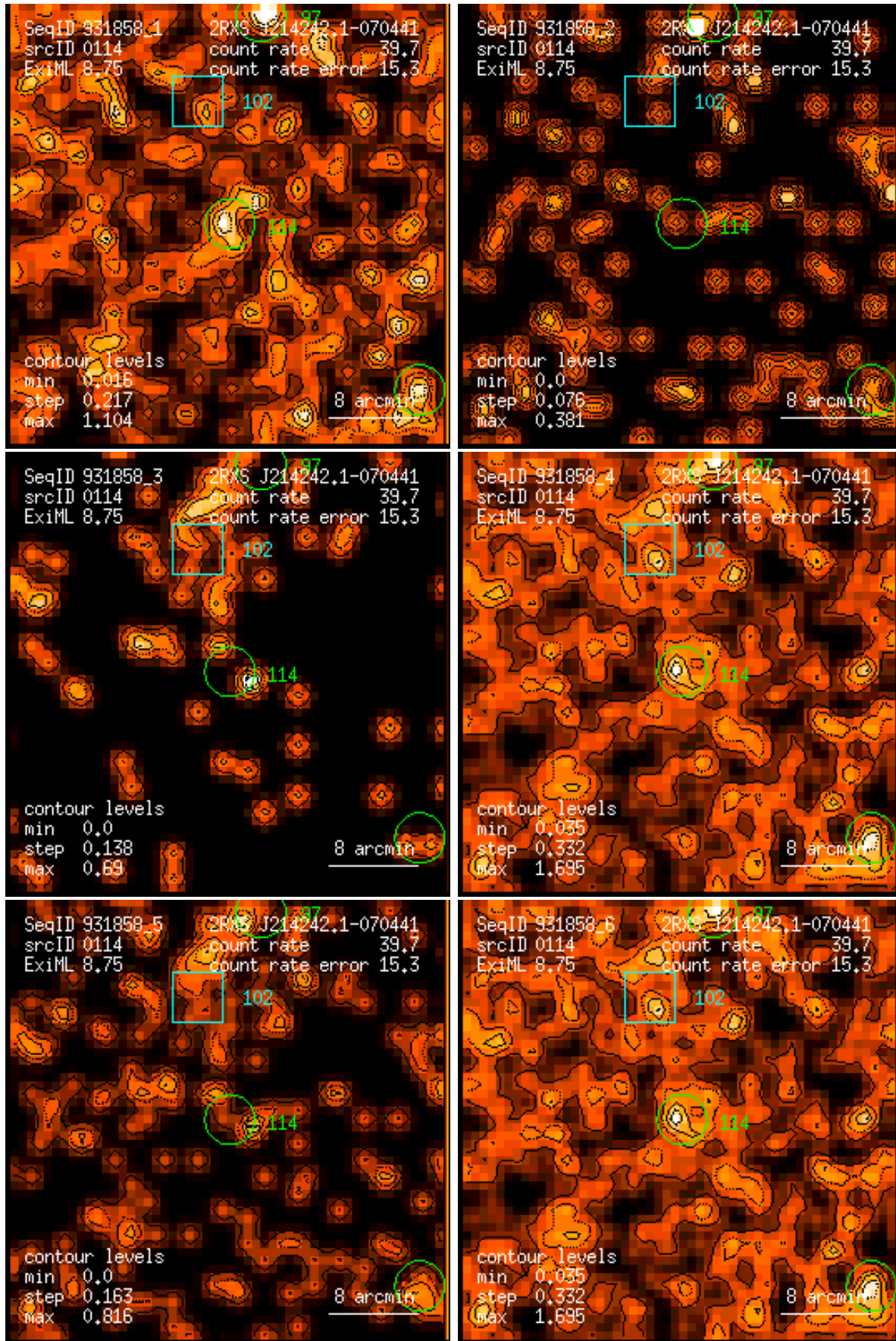
Figure 114: RASS 931858: detection 0114: band rate images, Gaussian filter: (1) PSPC channels 11 – 41, (2) 52 – 90, (3) 91 – 201, (4) 11 – 235, (5) 52 – 201, (6) 11 – 201. Broad band rates in counts/ks. Band rate contour levels in counts/ks/arcmin 2 .
