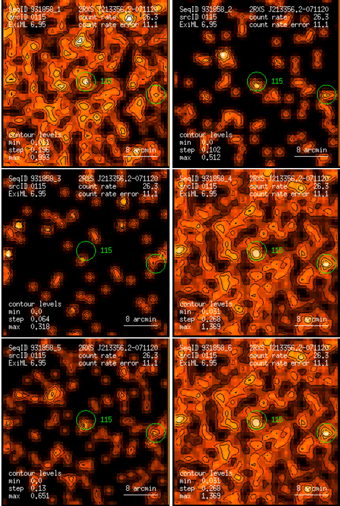
Figure 115: RASS 931858: detection 0115: band rate images, Gaussian filter: (1) PSPC channels 11 – 41, (2) 52 – 90, (3) 91 – 201, (4) 11 – 235, (5) 52 – 201, (6) 11 – 201. Broad band rates in counts/ks. Band rate contour levels in counts/ks/arcmin 2 .
