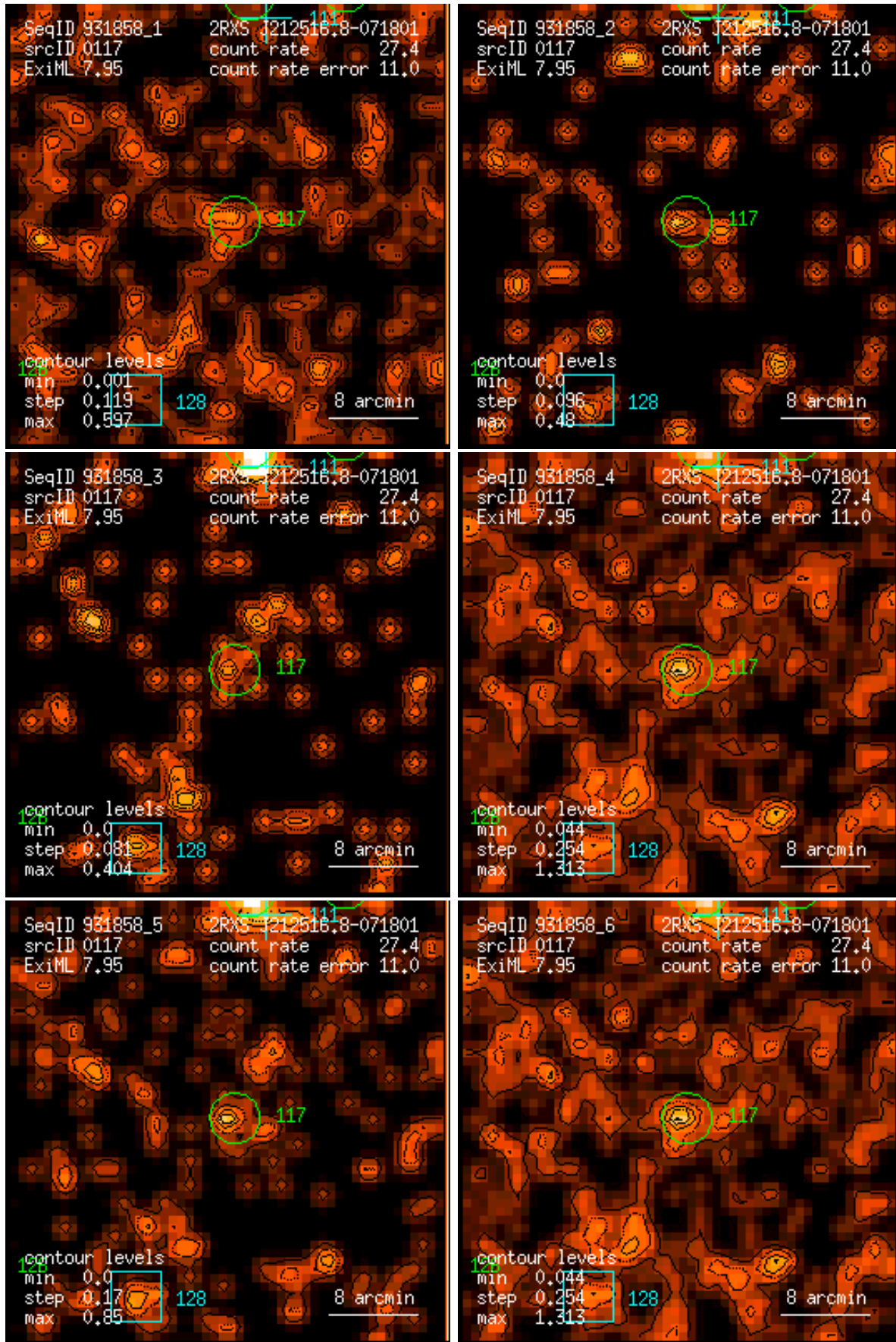
Figure 117: RASS 931858: detection 0117: band rate images, Gaussian filter: (1) PSPC channels 11 – 41, (2) 52 – 90, (3) 91 – 201, (4) 11 – 235, (5) 52 – 201, (6) 11 – 201. Broad band rates in counts/ks. Band rate contour levels in counts/ks/arcmin 2 .
