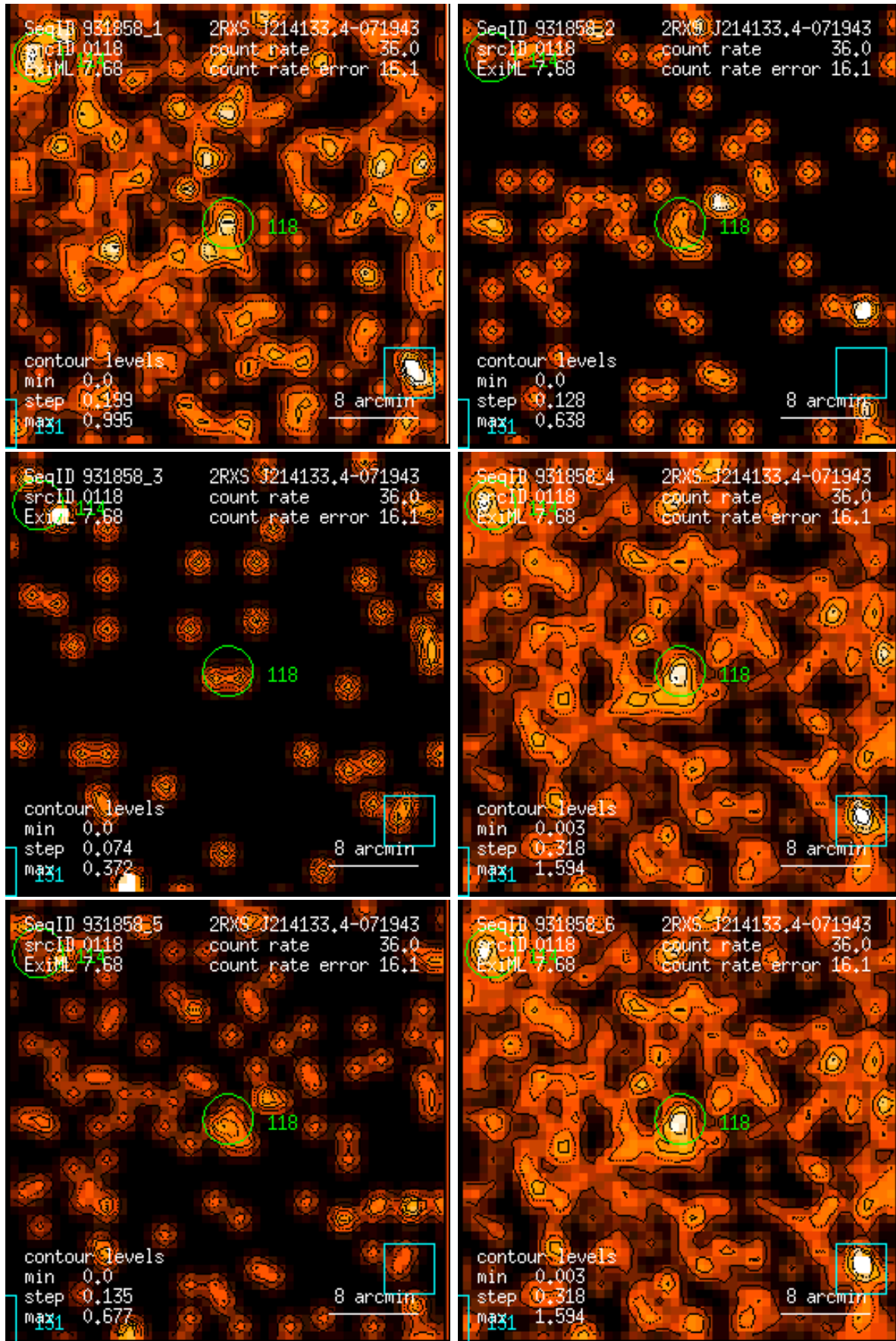
Figure 118: RASS 931858: detection 0118: band rate images, Gaussian filter: (1) PSPC channels 11 – 41, (2) 52 – 90, (3) 91 – 201, (4) 11 – 235, (5) 52 – 201, (6) 11 – 201. Broad band rates in counts/ks. Band rate contour levels in counts/ks/arcmin 2 .
