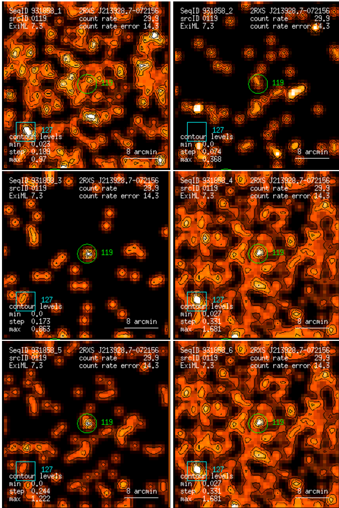
Figure 119: RASS 931858: detection 0119: band rate images, Gaussian filter: (1) PSPC channels 11 – 41, (2) 52 – 90, (3) 91 – 201, (4) 11 – 235, (5) 52 – 201, (6) 11 – 201. Broad band rates in counts/ks. Band rate contour levels in counts/ks/arcmin 2 .
