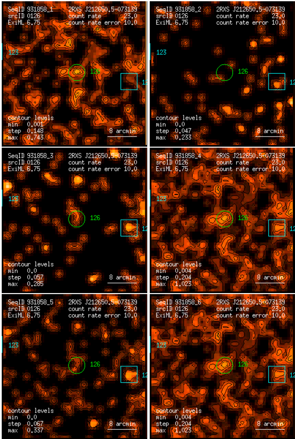
Figure 126: RASS 931858: detection 0126: band rate images, Gaussian filter: (1) PSPC channels 11 – 41, (2) 52 – 90, (3) 91 – 201, (4) 11 – 235, (5) 52 – 201, (6) 11 – 201. Broad band rates in counts/ks. Band rate contour levels in counts/ks/arcmin 2 .
