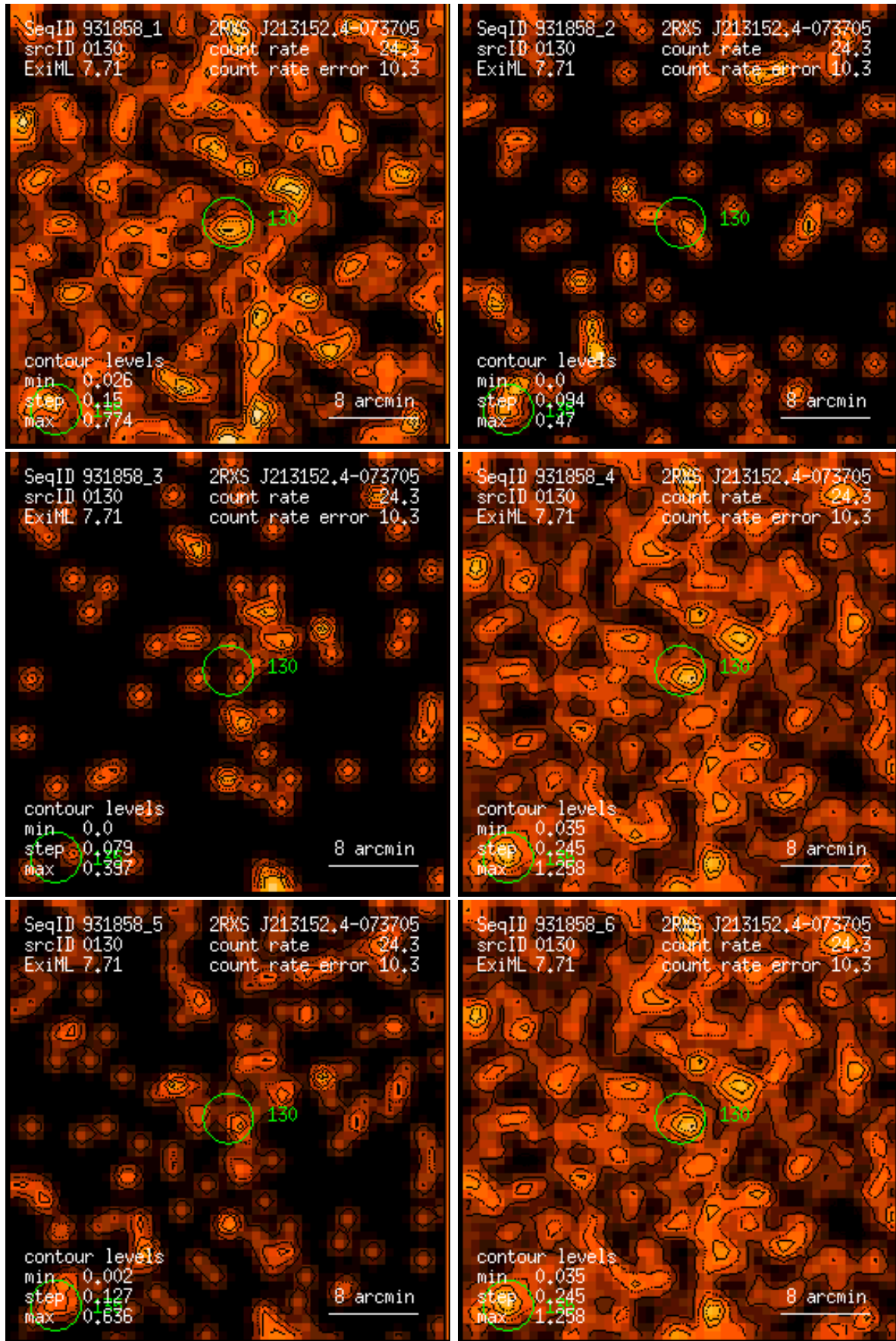
Figure 130: RASS 931858: detection 0130: band rate images, Gaussian filter: (1) PSPC channels 11 – 41, (2) 52 – 90, (3) 91 – 201, (4) 11 – 235, (5) 52 – 201, (6) 11 – 201. Broad band rates in counts/ks. Band rate contour levels in counts/ks/arcmin 2 .
