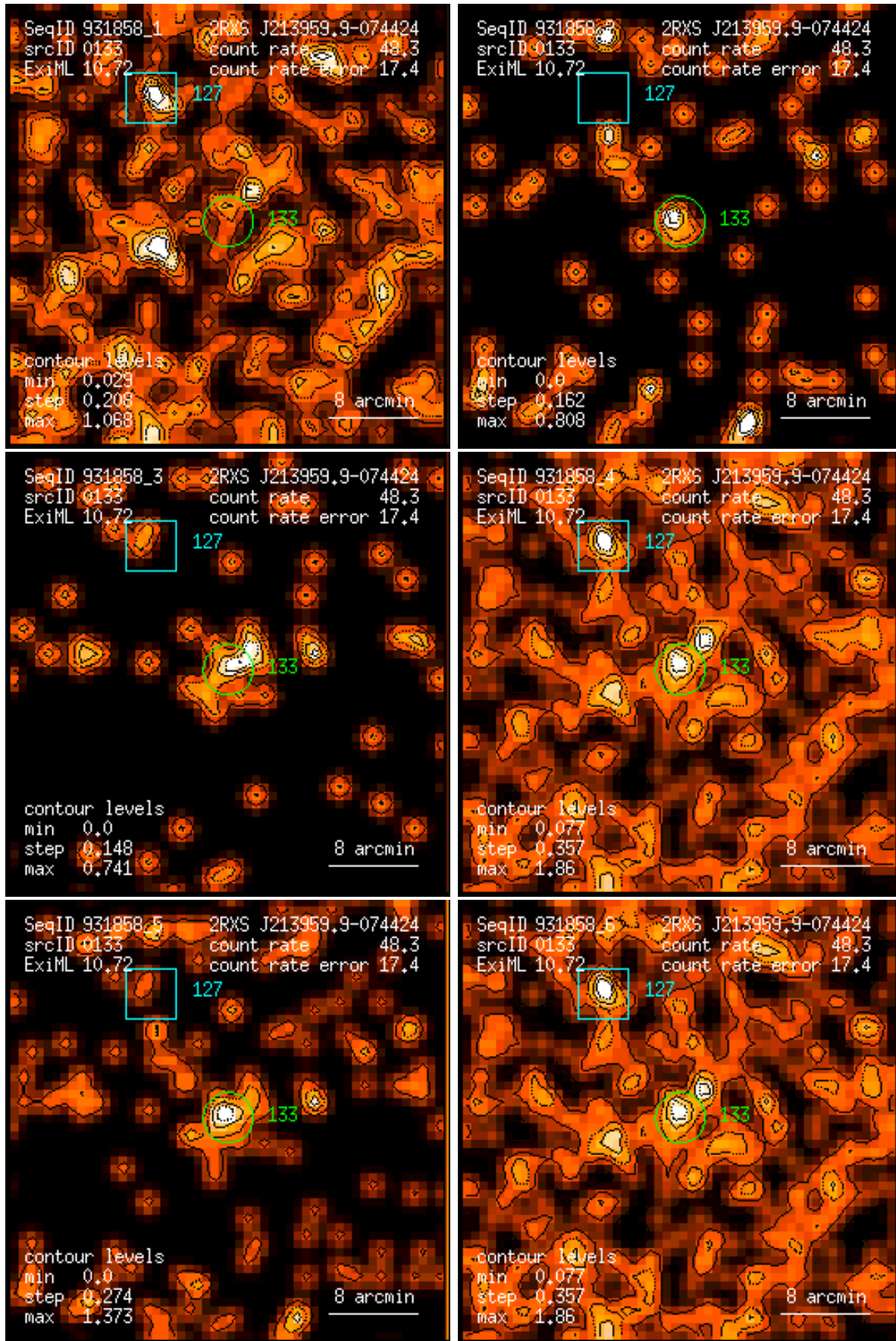
Figure 133: RASS 931858: detection 0133: band rate images, Gaussian filter: (1) PSPC channels 11 – 41, (2) 52 – 90, (3) 91 – 201, (4) 11 – 235, (5) 52 – 201, (6) 11 – 201. Broad band rates in counts/ks. Band rate contour levels in counts/ks/arcmin 2 .
