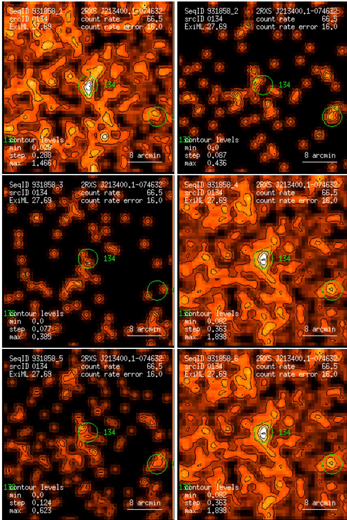
Figure 134: RASS 931858: detection 0134: band rate images, Gaussian filter: (1) PSPC channels 11 – 41, (2) 52 – 90, (3) 91 – 201, (4) 11 – 235, (5) 52 – 201, (6) 11 – 201. Broad band rates in counts/ks. Band rate contour levels in counts/ks/arcmin 2 .
