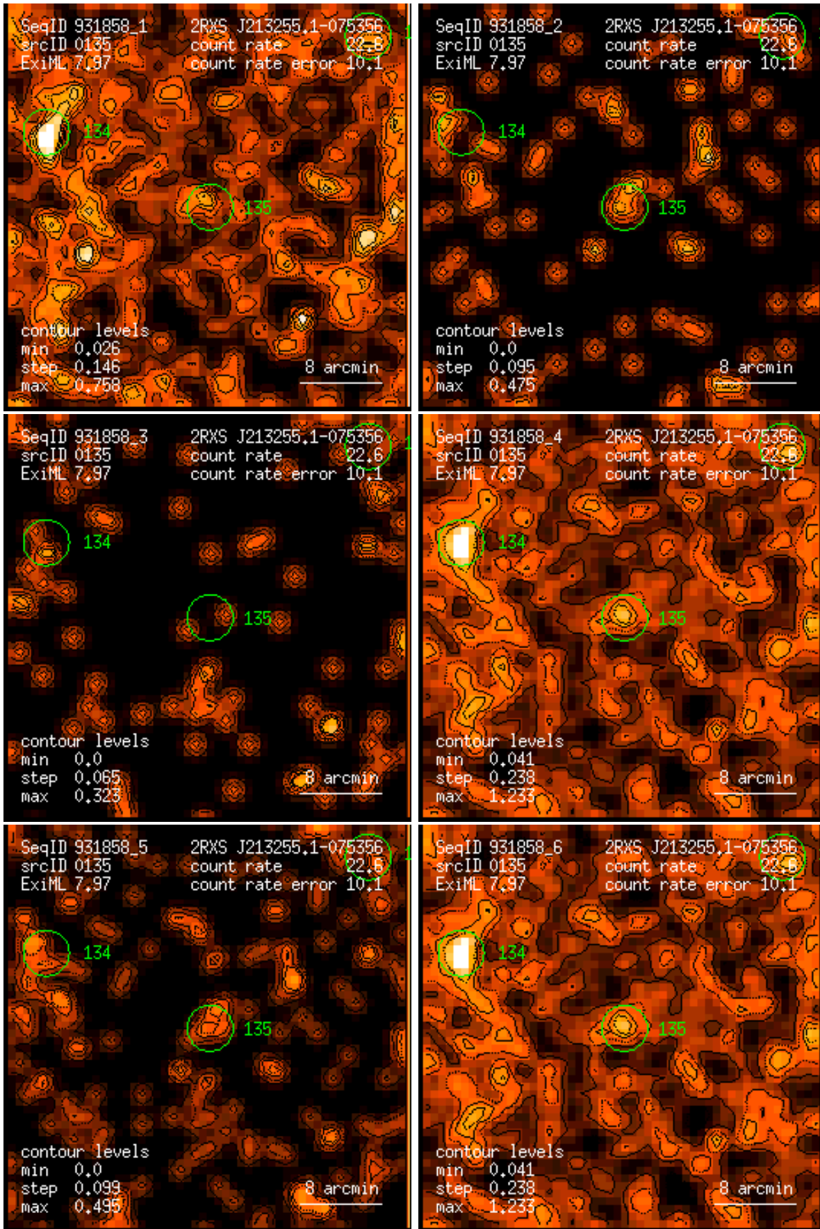
Figure 135: RASS 931858: detection 0135: band rate images, Gaussian filter: (1) PSPC channels 11 – 41, (2) 52 – 90, (3) 91 – 201, (4) 11 – 235, (5) 52 – 201, (6) 11 – 201. Broad band rates in counts/ks. Band rate contour levels in counts/ks/arcmin 2 .
