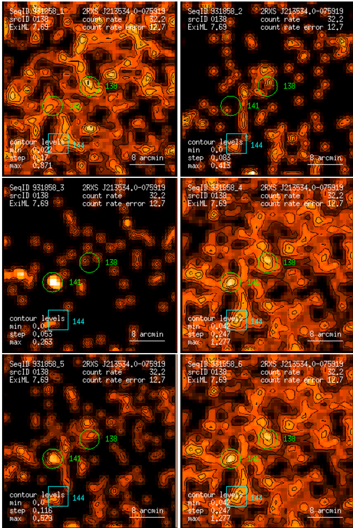
Figure 138: RASS 931858: detection 0138: band rate images, Gaussian filter: (1) PSPC channels 11 – 41, (2) 52 – 90, (3) 91 – 201, (4) 11 – 235, (5) 52 – 201, (6) 11 – 201. Broad band rates in counts/ks. Band rate contour levels in counts/ks/arcmin 2 .
