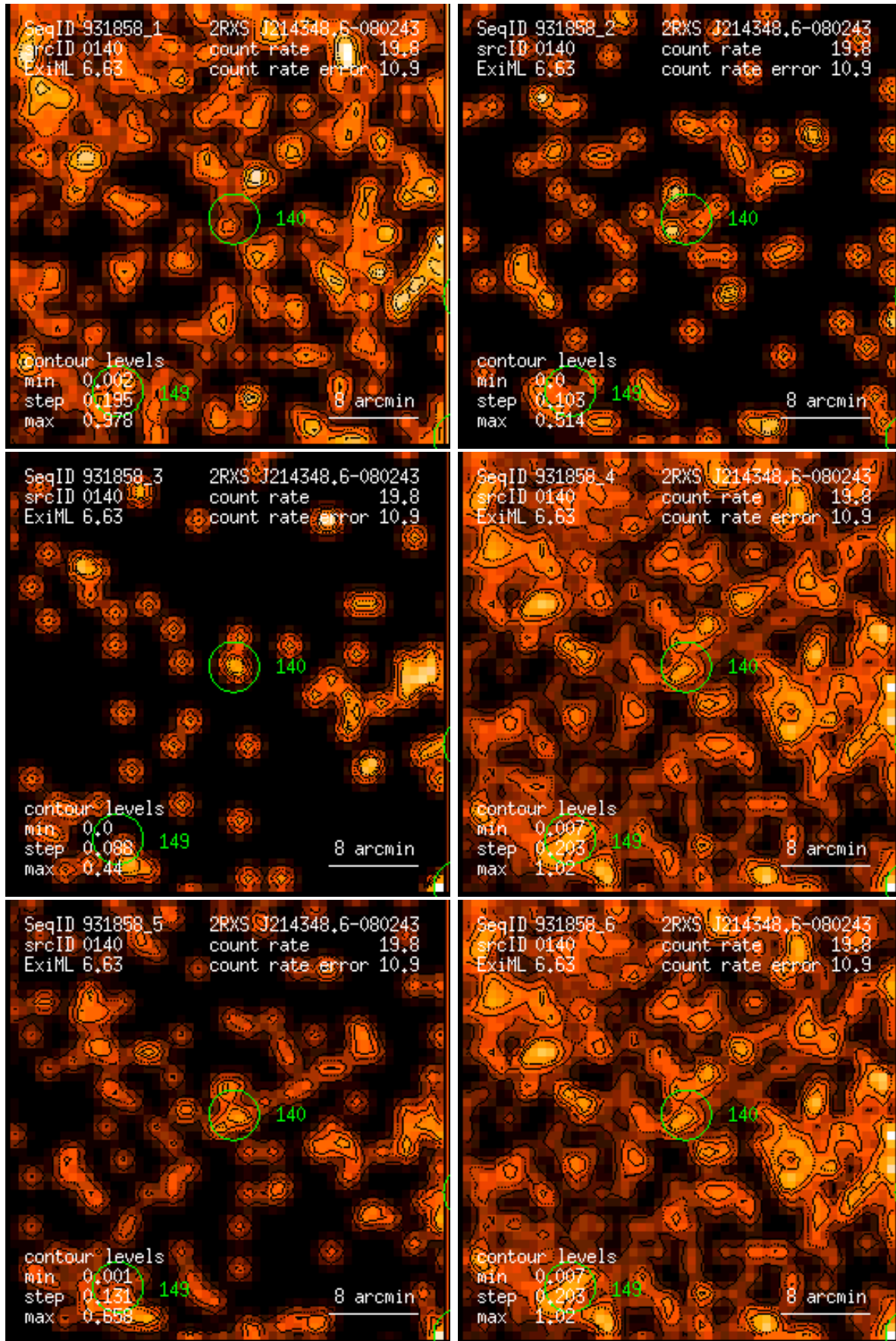
Figure 140: RASS 931858: detection 0140: band rate images, Gaussian filter: (1) PSPC channels 11 – 41, (2) 52 – 90, (3) 91 – 201, (4) 11 – 235, (5) 52 – 201, (6) 11 – 201. Broad band rates in counts/ks. Band rate contour levels in counts/ks/arcmin 2 .
