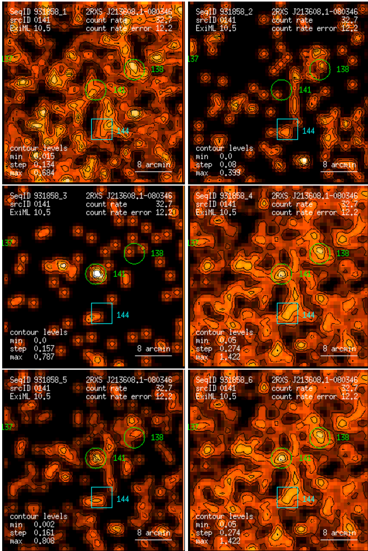
Figure 141: RASS 931858: detection 0141: band rate images, Gaussian filter: (1) PSPC channels 11 – 41, (2) 52 – 90, (3) 91 – 201, (4) 11 – 235, (5) 52 – 201, (6) 11 – 201. Broad band rates in counts/ks. Band rate contour levels in counts/ks/arcmin 2 .
