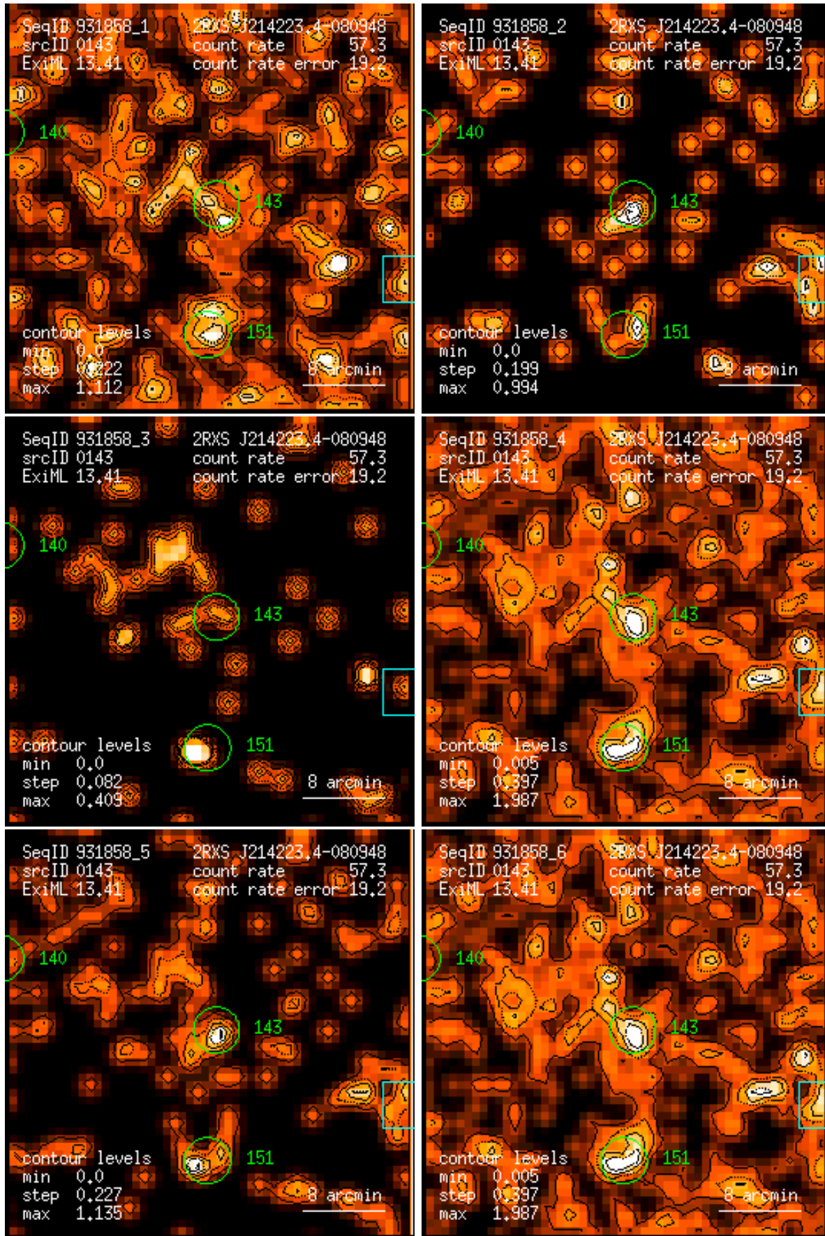
Figure 143: RASS 931858: detection 0143: band rate images, Gaussian filter: (1) PSPC channels 11 – 41, (2) 52 – 90, (3) 91 – 201, (4) 11 – 235, (5) 52 – 201, (6) 11 – 201. Broad band rates in counts/ks. Band rate contour levels in counts/ks/arcmin 2 .
