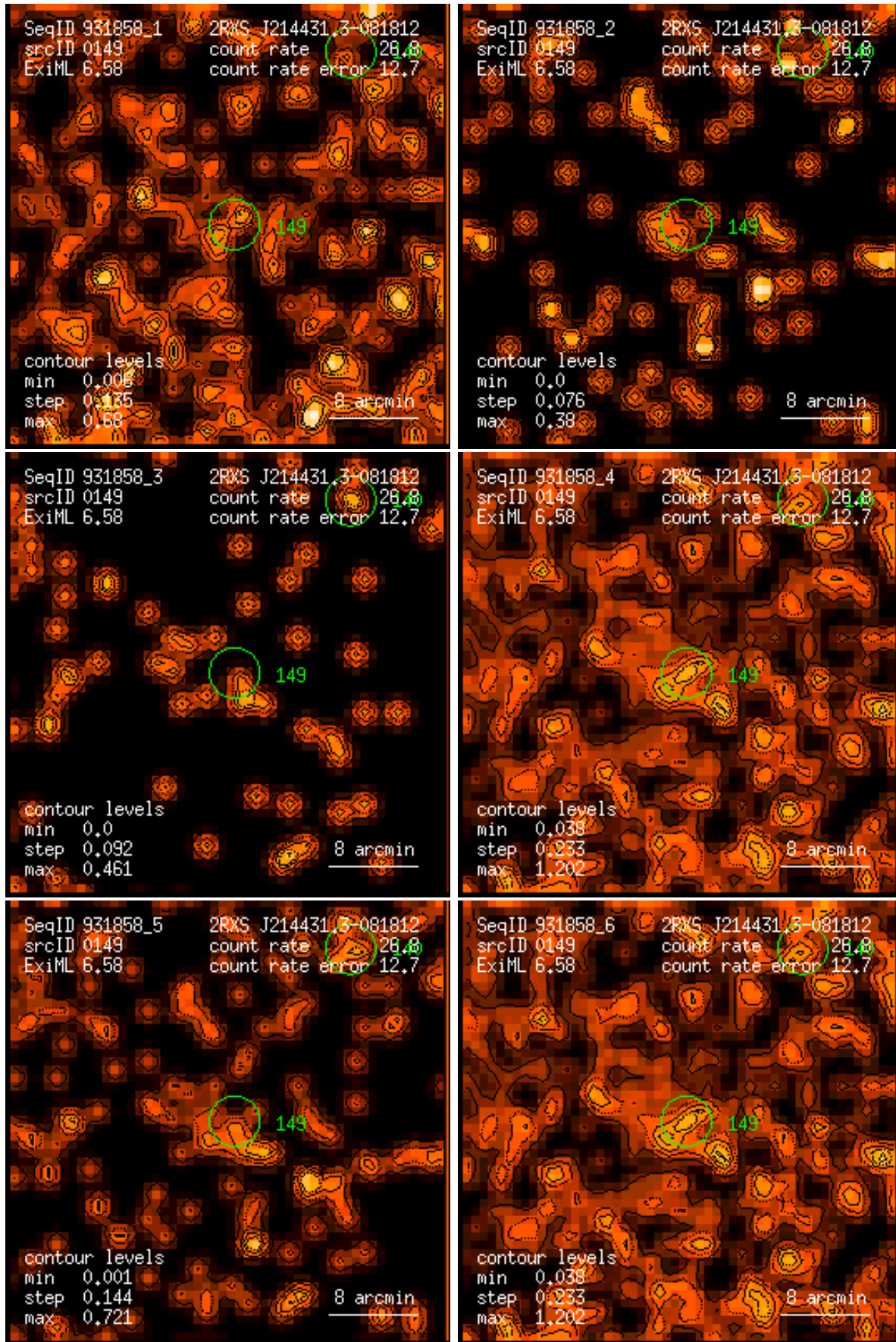
Figure 149: RASS 931858: detection 0149: band rate images, Gaussian filter: (1) PSPC channels 11 – 41, (2) 52 – 90, (3) 91 – 201, (4) 11 – 235, (5) 52 – 201, (6) 11 – 201. Broad band rates in counts/ks. Band rate contour levels in counts/ks/arcmin 2 .
