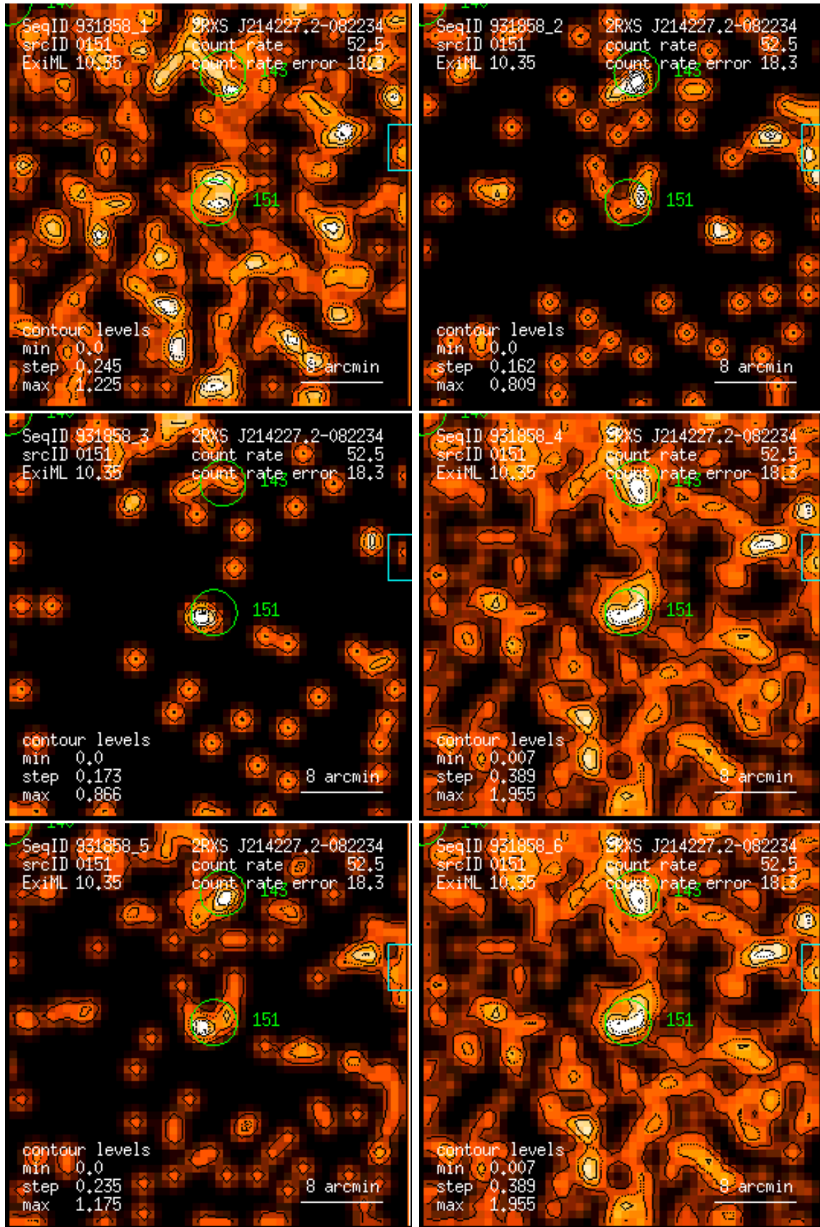
Figure 151: RASS 931858: detection 0151: band rate images, Gaussian filter: (1) PSPC channels 11 – 41, (2) 52 – 90, (3) 91 – 201, (4) 11 – 235, (5) 52 – 201, (6) 11 – 201. Broad band rates in counts/ks. Band rate contour levels in counts/ks/arcmin 2 .
