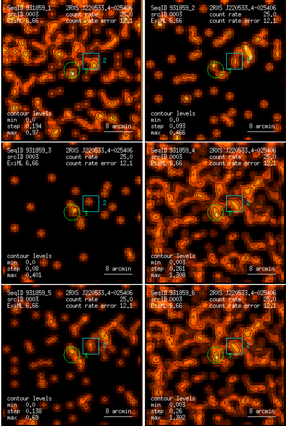
Figure 3: RASS 931859: detection 0003: band rate images, Gaussian filter: (1) PSPC channels 11 – 41, (2) 52 – 90, (3) 91 – 201, (4) 11 – 235, (5) 52 – 201, (6) 11 – 201. Broad band rates in counts/ks. Band rate contour levels in counts/ks/arcmin 2 .
