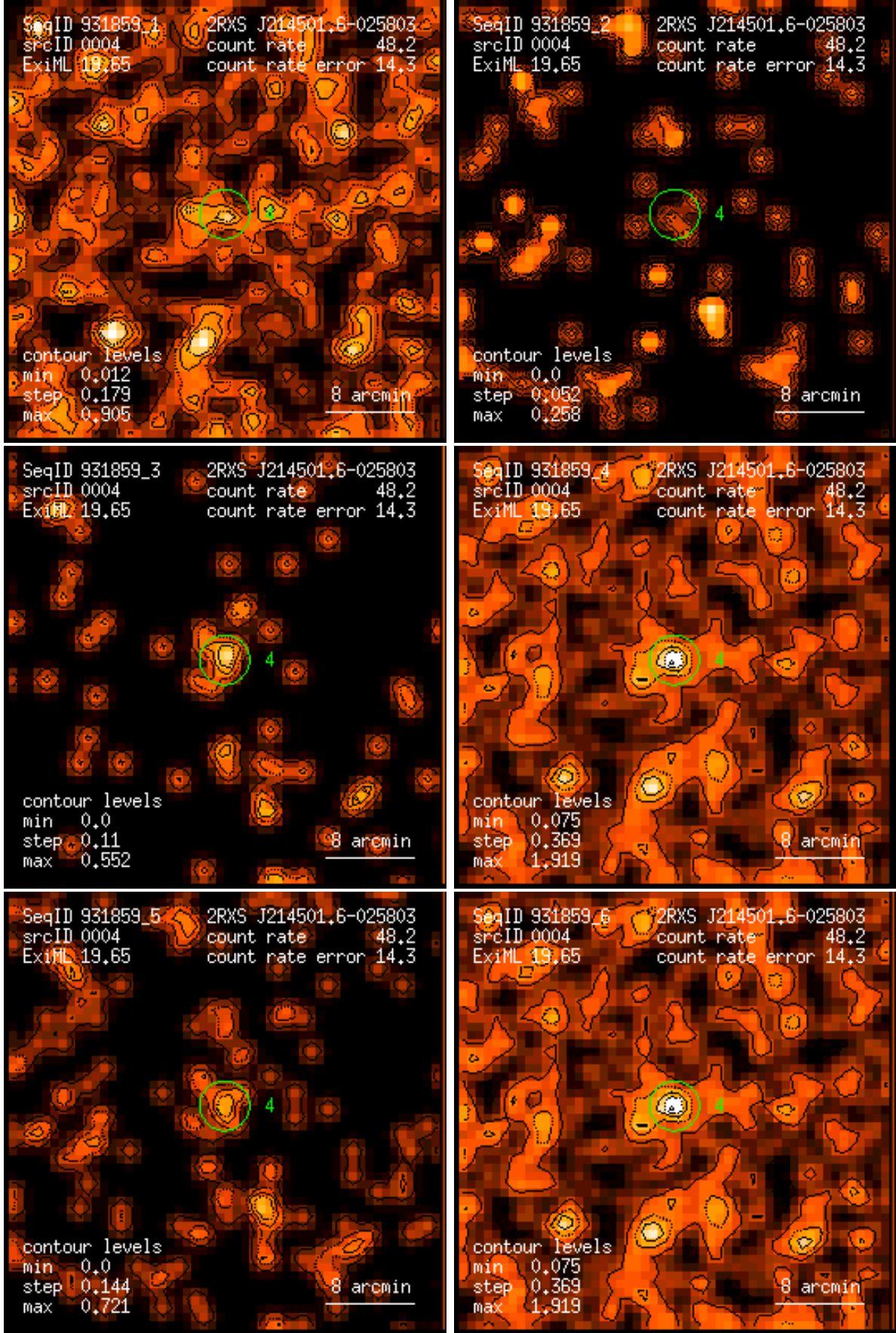
Figure 4: RASS 931859: detection 0004: band rate images, Gaussian filter: (1) PSPC channels 11 – 41, (2) 52 – 90, (3) 91 – 201, (4) 11 – 235, (5) 52 – 201, (6) 11 – 201. Broad band rates in counts/ks. Band rate contour levels in counts/ks/arcmin 2 .
