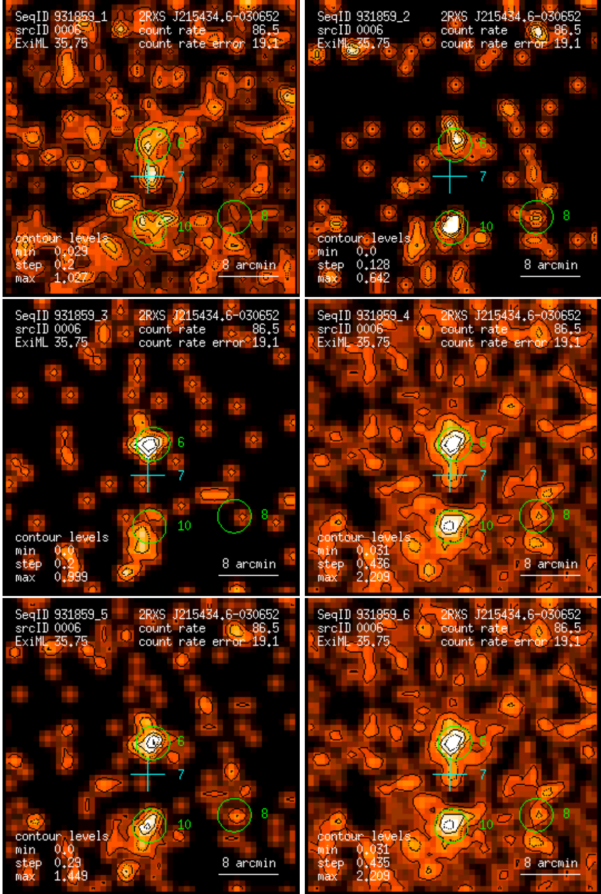
Figure 6: RASS 931859: detection 0006: band rate images, Gaussian filter: (1) PSPC channels 11 – 41, (2) 52 – 90, (3) 91 – 201, (4) 11 – 235, (5) 52 – 201, (6) 11 – 201. Broad band rates in counts/ks. Band rate contour levels in counts/ks/arcmin 2 .
